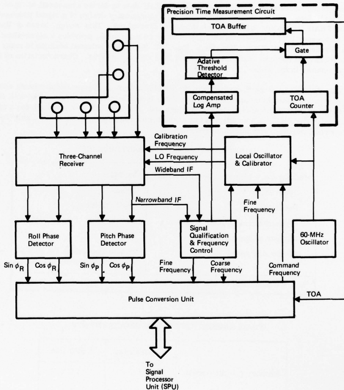
Passive Range Interferometer Sensor (PRAIS)
