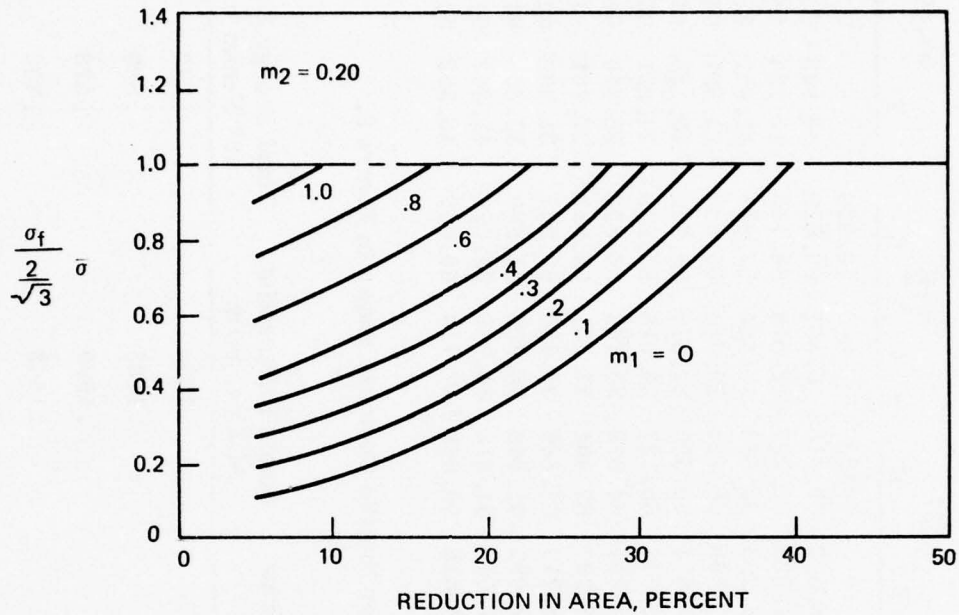
Figure 3. Drawing Limit Diagram for a Constant Friction at the Punch-Material Interface ( R_0 = 70 mm, r_0 = 43 mm, Temperature = 20° C, Curved-Straight-Curved Die Angle = 17.8 Degrees)
