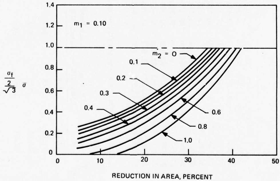
Figure 4. Drawing Limit Diagram for a Constant Friction at the Die-Material Interface ( R_0 = 70 mm, r_0 = 43 mm, Temperature = 20° C, Curved-Straight-Curved Die Angle = 17.8 Degrees)
