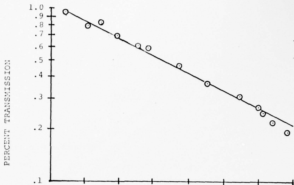
Figure 15. CW CO 2 (R(14) (10.288 \mu m) absorption in NH 3
