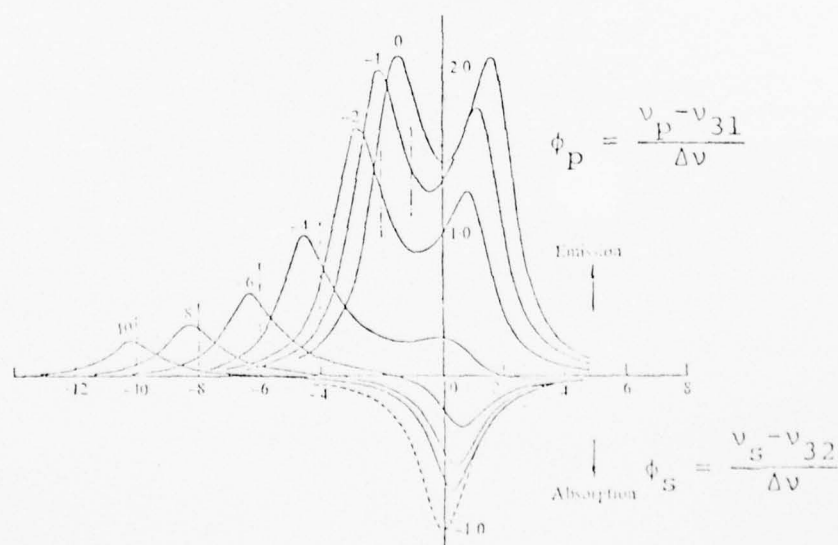
Figure 18. Theoretical shapes of the signal line under resonant and off-resonant pumping with w_p = 3 in a three-level system, where \nu_{31}/\nu_{32} = 9.47 and \phi_p = \nu_p - \nu_{31}/\Delta\nu . 14
