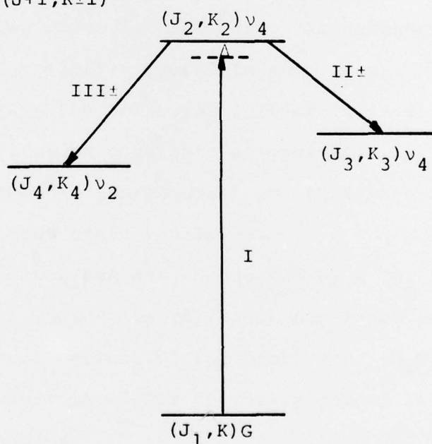
Figure 24. Optically pumped PH 3 possibilities. II. the \nu_4 band.
