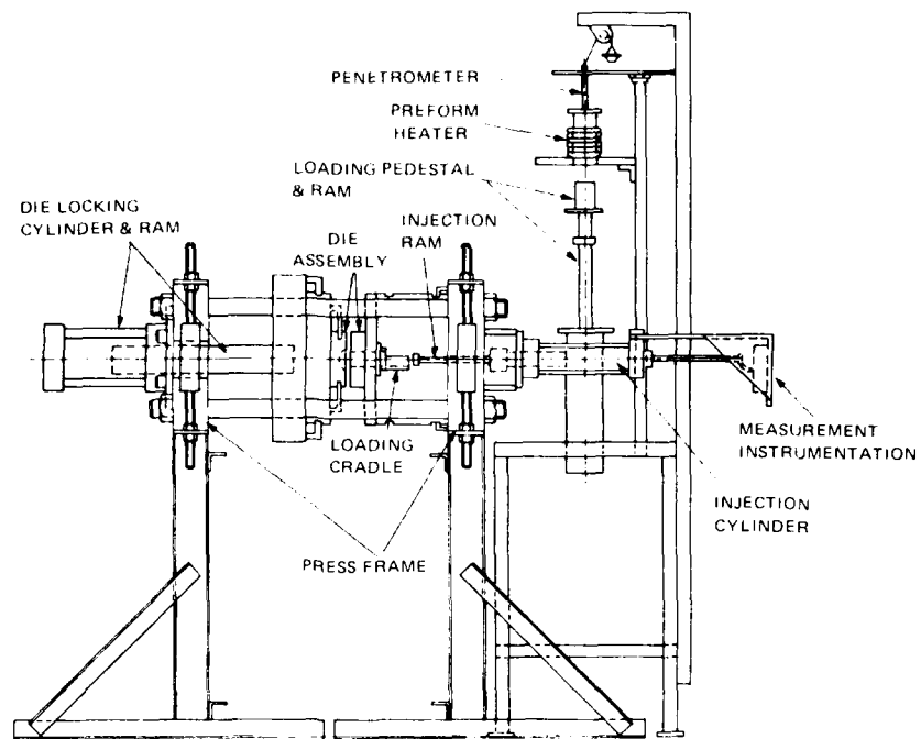
Figure 4 Schematic of Machine Casting Unit
