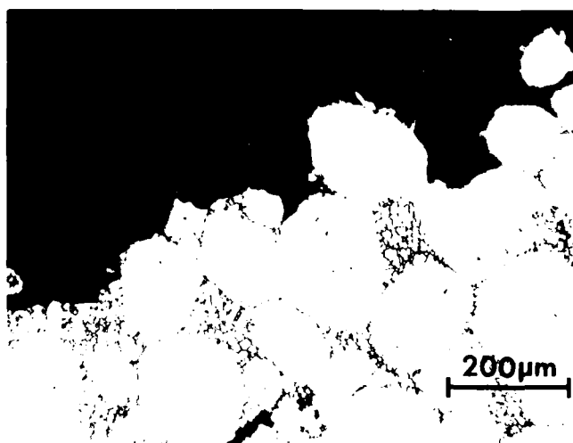
Figure 20 Appearance of the Room Temperature Tensile Fracture of a Machine Thixocast Simulated Airfoil Section. A) Topographic Feature on Fracture Surface, and B) Longitudinal Section Which Includes Fracture Surface
