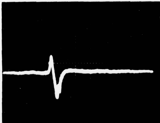
Fig. 33 Screen Ingestion Nickel, Buckshot, and Aluminum Oxide
