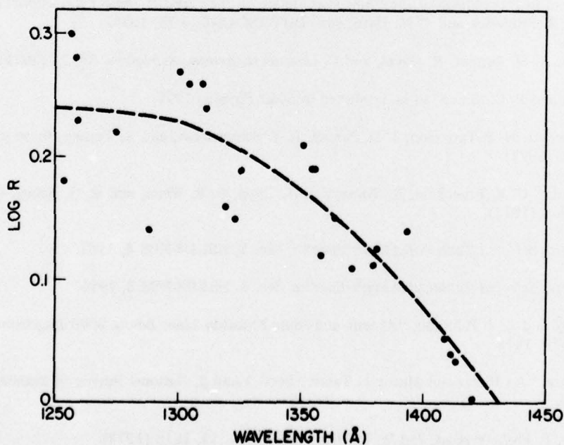
Fig. 4 - Ratio of intensities, reflight instrument, to CALROC.
