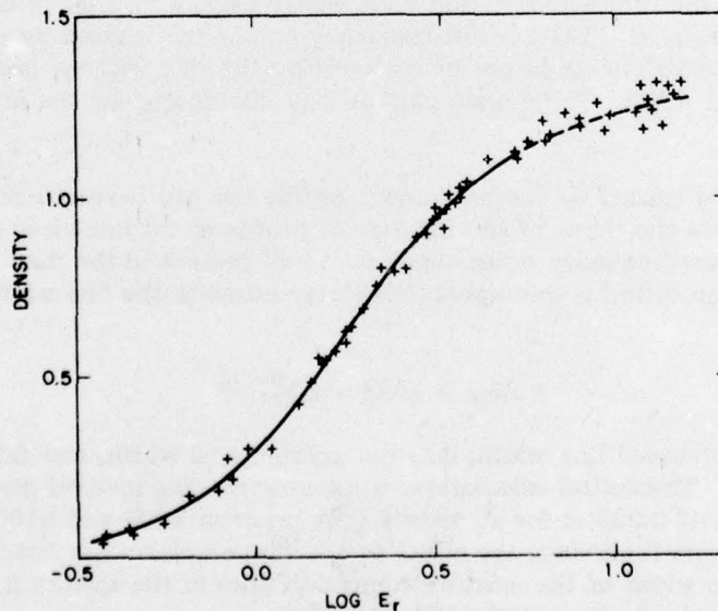
Fig. 3 — Example of film characteristic curve determined from the flight exposures. Crosses mark the observed points shifted along the exposure axis to form the best possible average curve.
