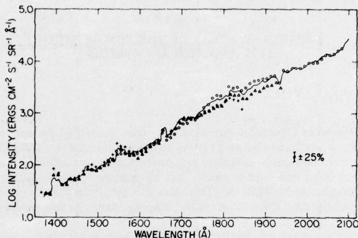
Fig. 1 — Comparison of solar mean intensities averaged over 10 Å intervals. The full line represent the NRL CALROC data used in the atlas. Open circles are the observations of Samain and Simon [10], crosses the observations of Rottman [6], and triangles the observations of Heroux and Swirbalus [7].
