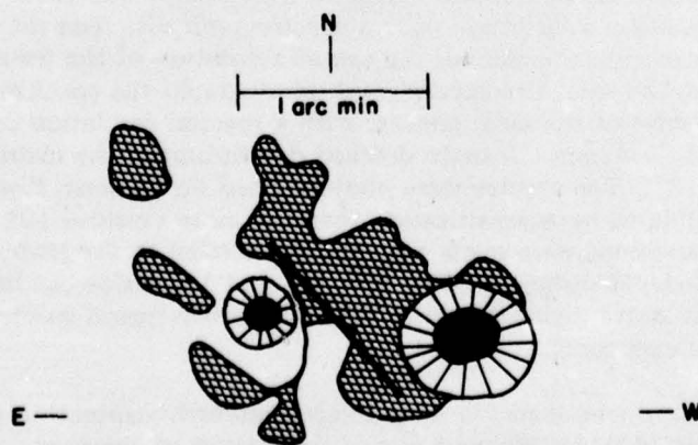
Fig. 2 — Position of the spectrograph slit inside active region McMath 508 on September 4, 1973.
