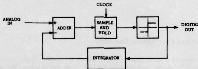
Fig. 1 — Basic delta modulator
