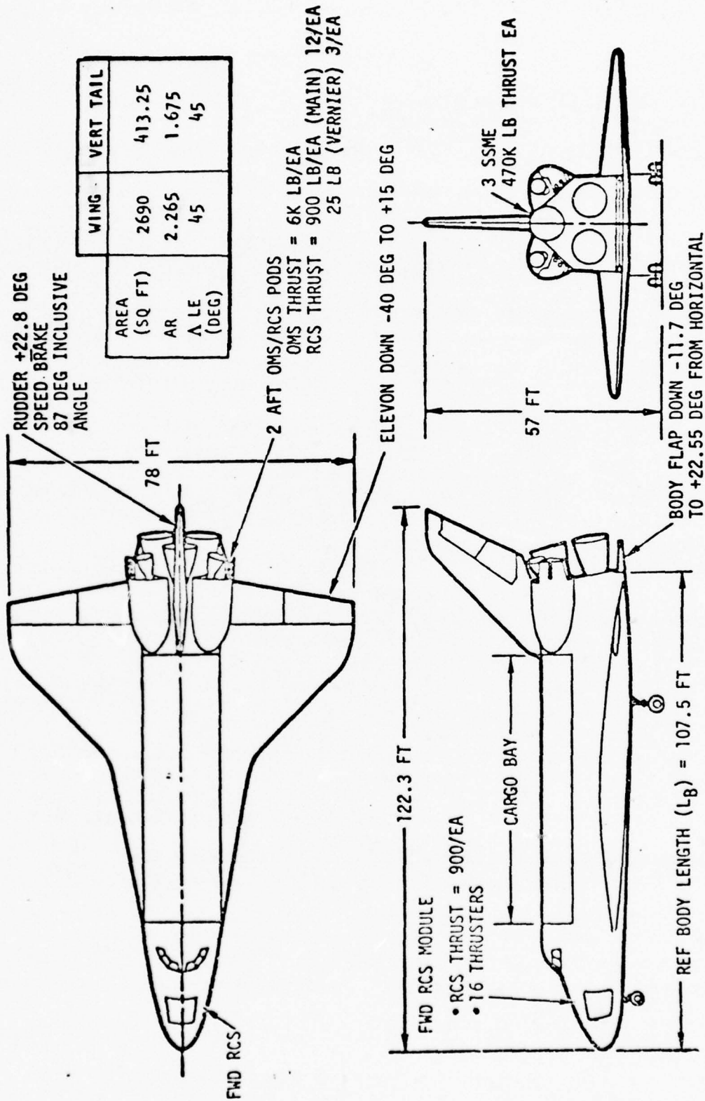
Figure II-2. Shuttle Orbiter
