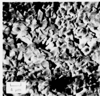
(c) 45% POROUS SINTERED ALUMINA
