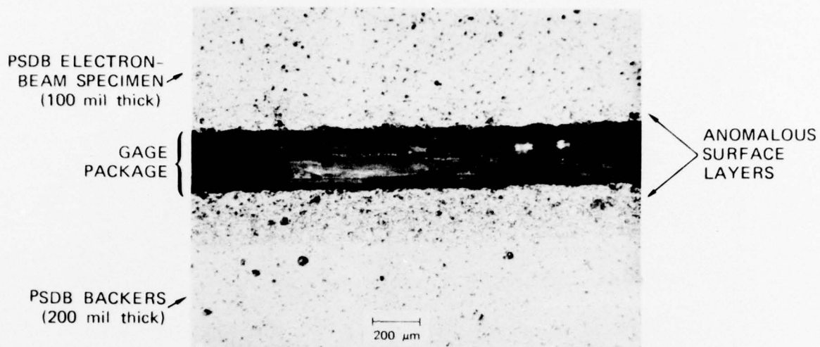
(a) ELECTRON-BEAM EXPERIMENT 4
