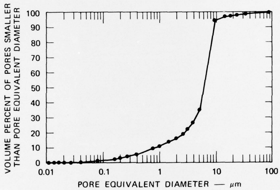
FIGURE 2 PORE SIZE DISTRIBUTION FOR 22% POROUS SINTERED ALUMINA
