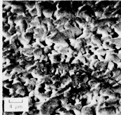
(b) 36% POROUS SINTERED ALUMINA
