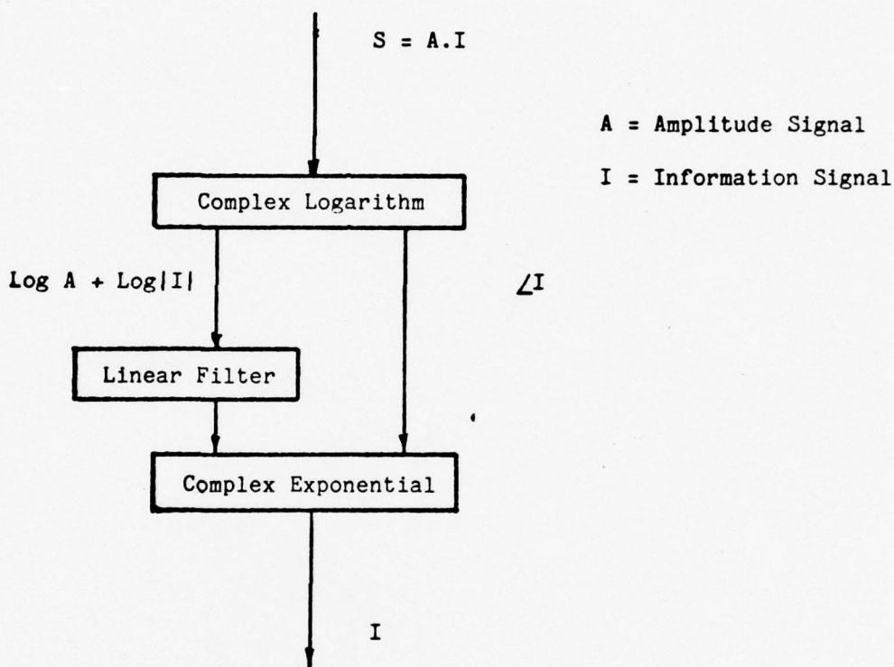
Figure 13 -- Homomorphic AGC element
