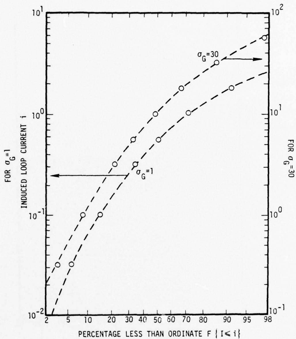
Figure 5(a). Probability Distributions of the Induced Loop Currents I for the Two-Dimensional Case of Equally Probable Area ( A, 2d ) and Equally Probable Radius ( R, 2d ) with Size Parameter \alpha = 1 and Mutual Coupling Strength \sigma_G = 1 and \sigma_G = 30
