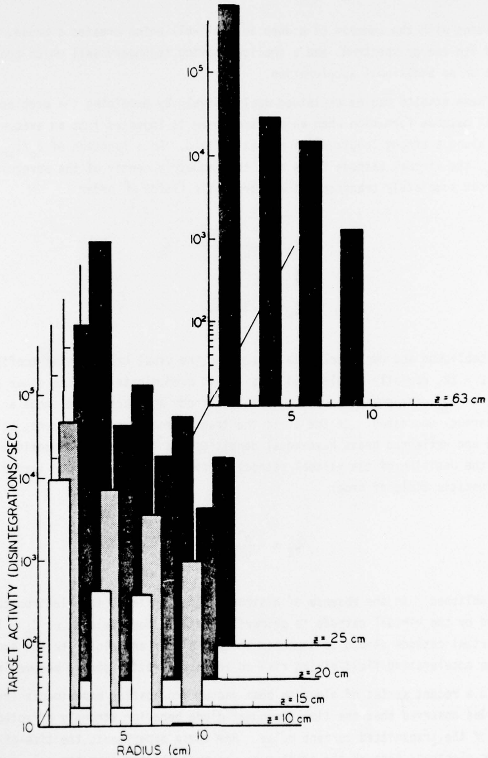
Figure 3. Carbon Target Activation as a Function of Radial Distance From the Axis of the Drift Chamber and Longitudinal Distance From the Anode at 240 mTorr of Deuterium for I_0/I_{s0} = 2.2 .
