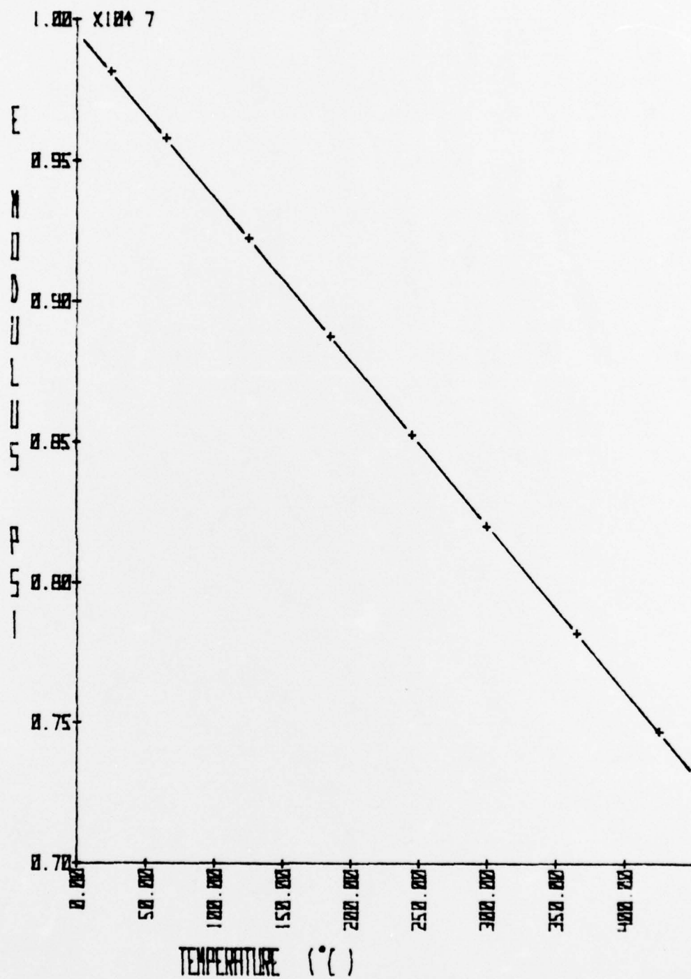
Figure 24 - ELASTIC MODULUS (E) VS. TEMPERATURE, (11).
