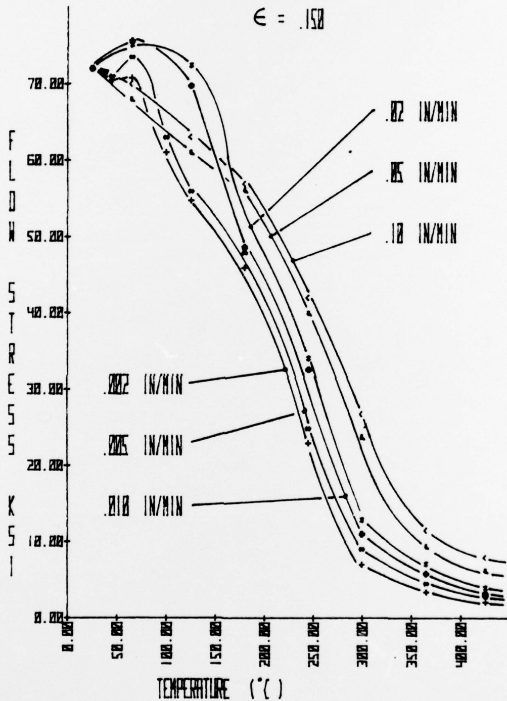
Figure 22 - FLOW STRESS VS. TEMPERATURE AT A TRUE STRAIN OF 0.15 FOR SIX STRAIN RATES.
