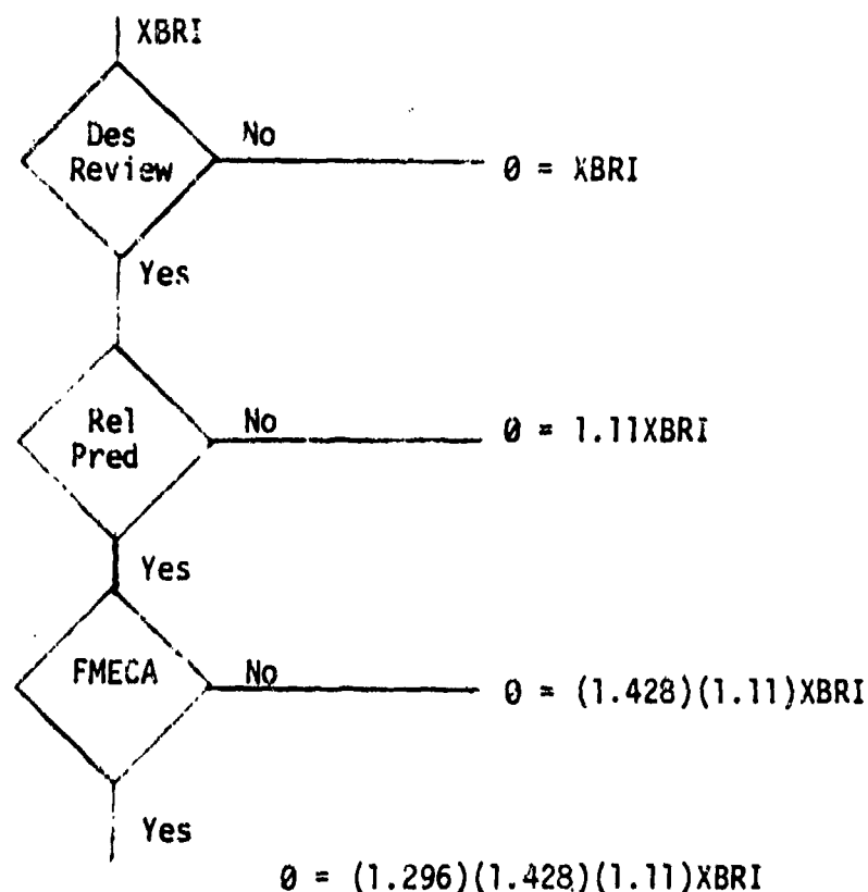
Figure A3. Flow Chart of Design Review, Prediction and FMECA Programs
