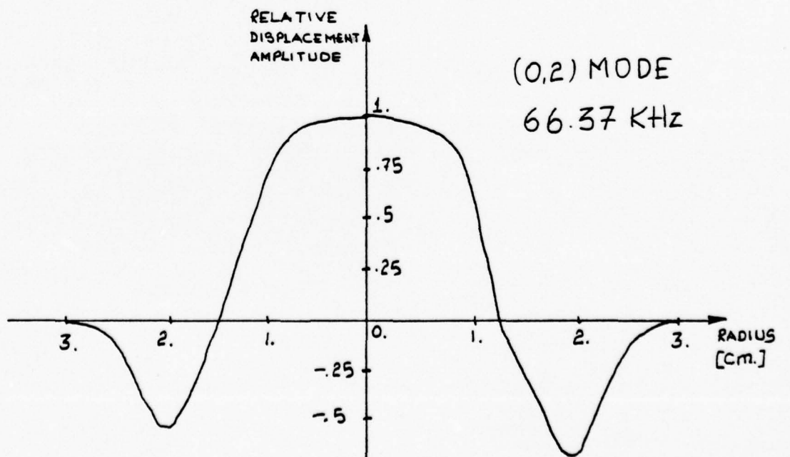
Figure 8 - RELATIVE DISPLACEMENT AMPLITUDES
