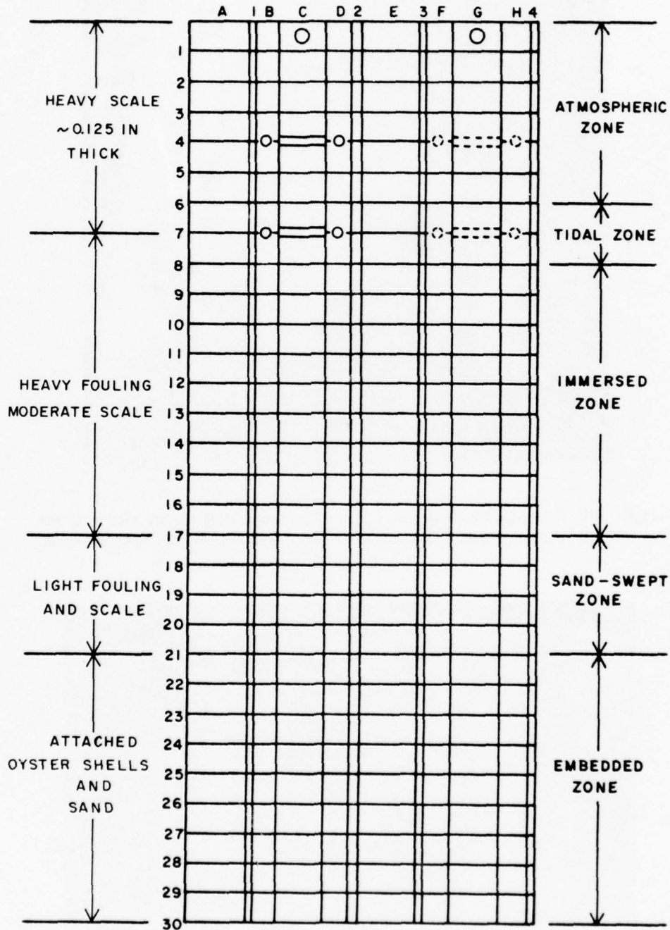
PILE NO. 1C BARE CARBON STEEL
