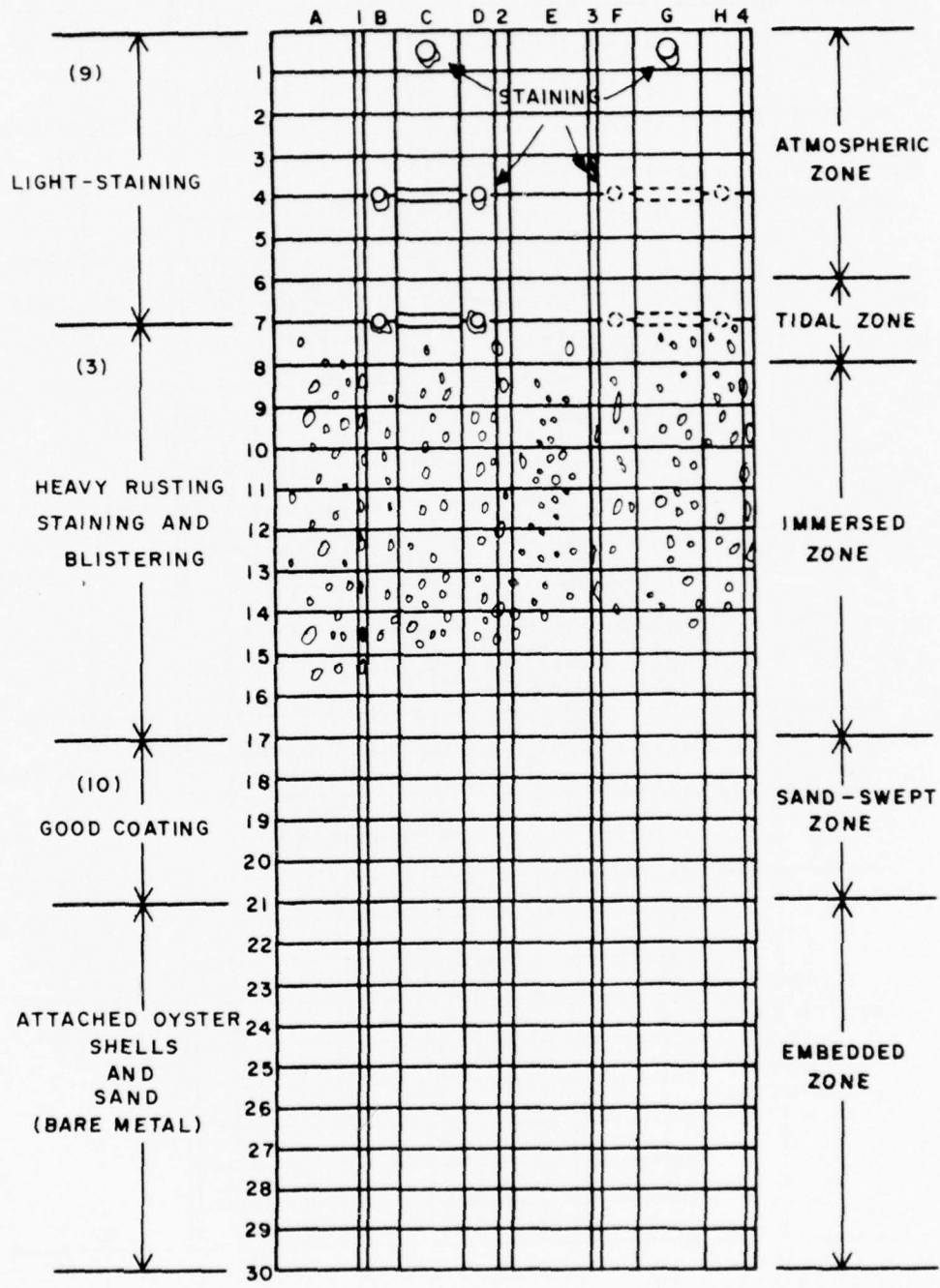
PILE NO. 8C ALUMINUM PIGMENTED EPOXY-TAR ON CARBON STEEL
