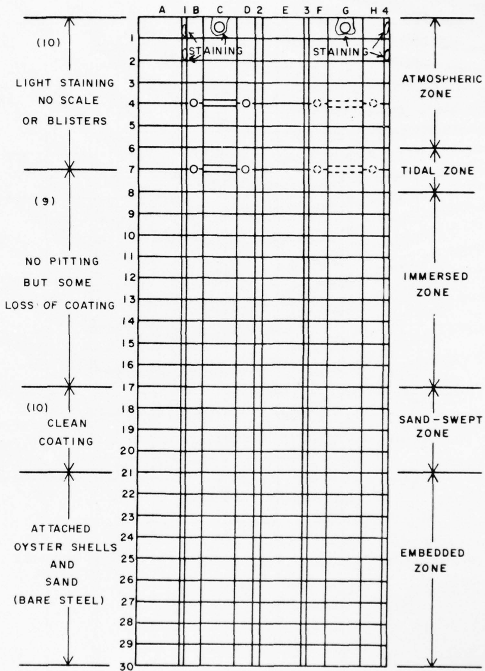
PILE NO. 5C COAL TAR EPOXY ON CARBON STEEL WITH ZINC ANODES
