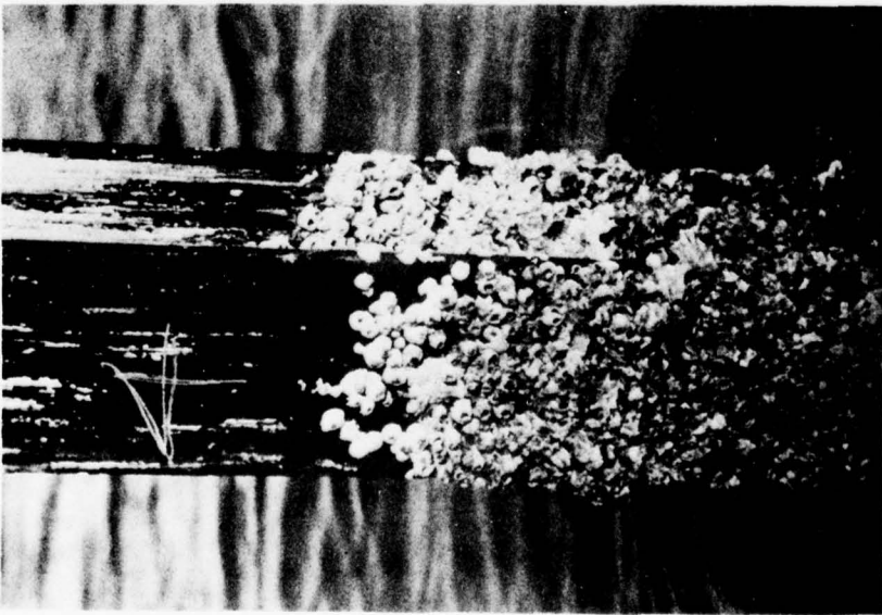
Figure A4. Coal-tar epoxy (C-200) on carbon steel. Photograph of upper immersed and lower atmospheric zones indicates the degree of marine fouling. Some damage to the flanges is also evident.
