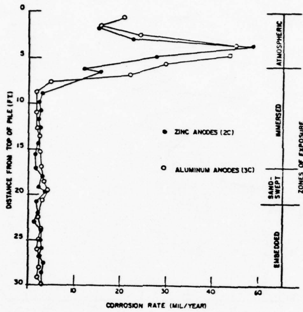
Figure 17. Corrosion profile of cathodically protected bare carbon steel. SI conversion factors: 1 ft = 0.3048 m; 1 mil = 0.0254 mm.
