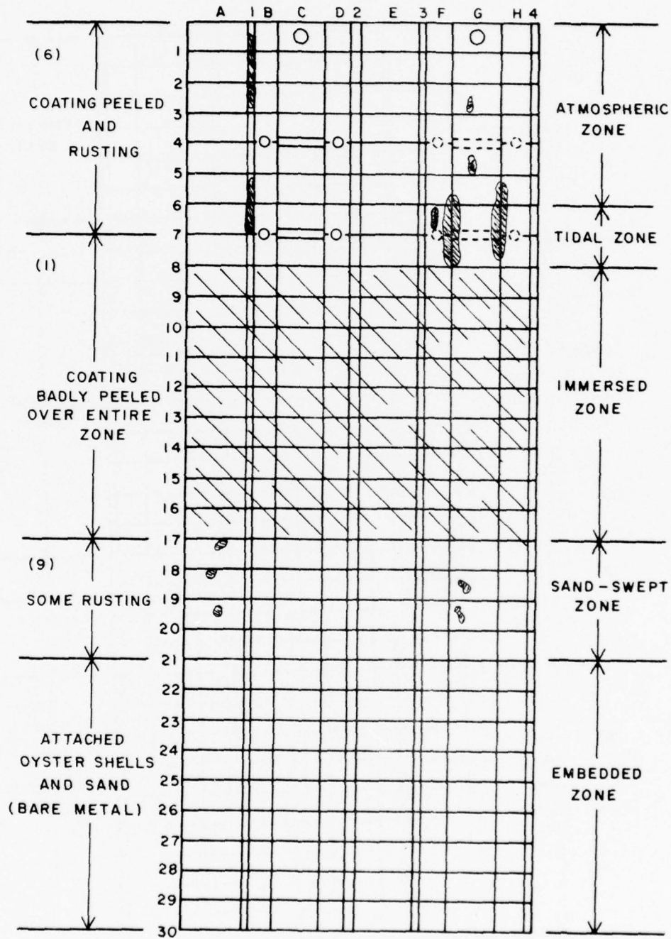
PILE NO. IIC EPOXY OVER INORGANIC ZINC PRIMER ON CARBON STEEL
