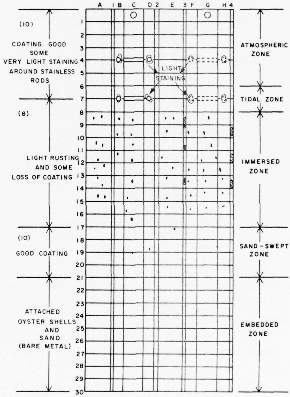
PILE NO. 9C ALUMINUM PIGMENTED COAL TAR (TARSET) EPOXY ON CARBON STEEL
