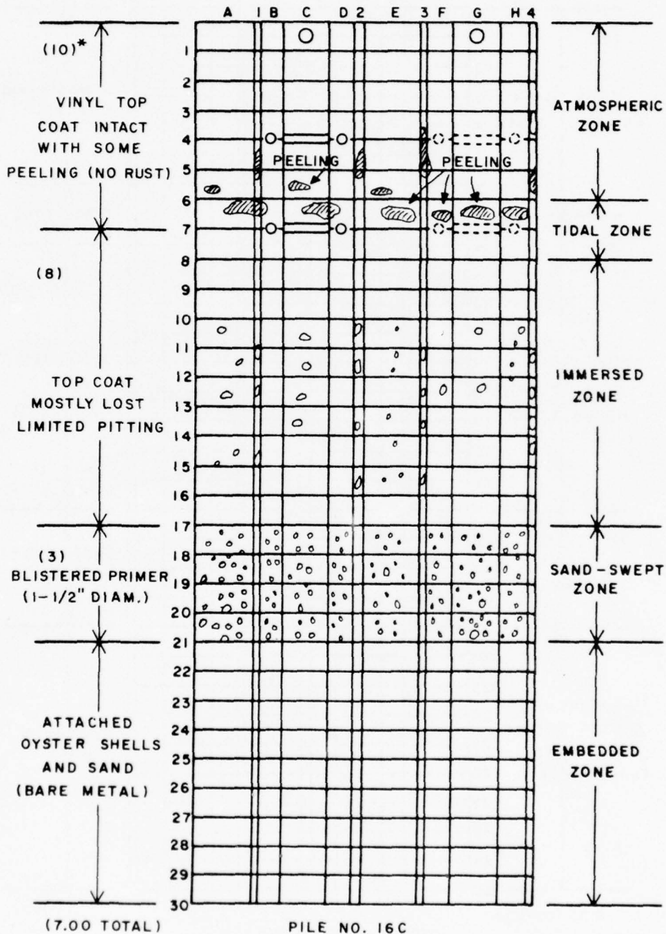
PILE NO. 16C FLAME-SPRAYED ZINC WITH NAVY VINYL TOPCOAT *TOPCOAT HAD PEELED BUT NO RUST WAS PRESENT
