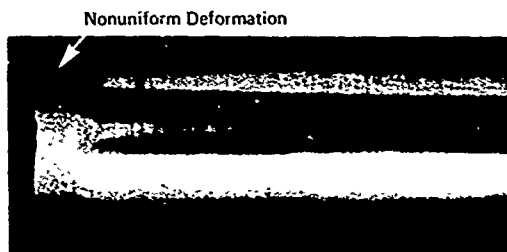
Figure 3. Localized torsional deformation of 18Ni (200) maraging steel as a result of monotonic loading. Mag. 4X.
