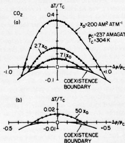
FIG. 2. Contours of constant susceptibility in \text{CO}_2 . Data are from Ref. 10. The solid lines are empirically determined fits to the data (Refs. 11, 19). Note the expanded scales used in Fig. 2(b).
