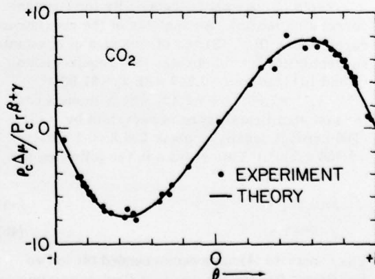
FIG. 4. Dependence of the chemical potential on \theta (density) at constant \nu . Data are from Ref. 17, plotted for T_c = 31.00^\circ\text{C} . The solid curve corresponds to Eq. (B1c).
