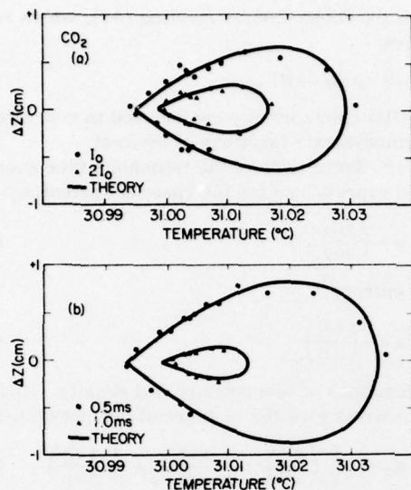
FIG. 8. Contours of constant wave scattering: (a) intensity; (b) inverse Rayleigh linewidth. Solid curves are contours of constant r , plotted for T_c = 31.0027^\circ\text{C} . Values of r have been assigned arbitrarily in (a) and have been set equal to (\tau/\tau_0)^{-1/\nu} in (b), with \tau_0 = 1.55 \mu\text{sec} , \nu = 0.63 .
