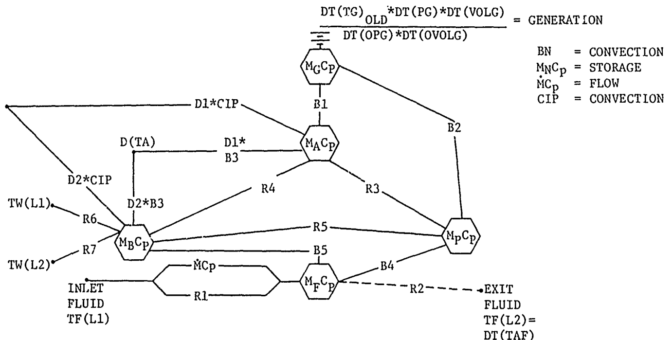
FIGURE 6.71-3 THERMAL MODEL
