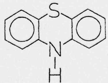
PHENOTHIAZINE
