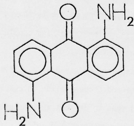
1,5-DAAQ
