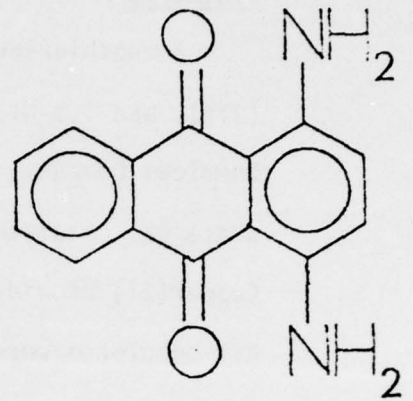
1,4-DAAQ ™
