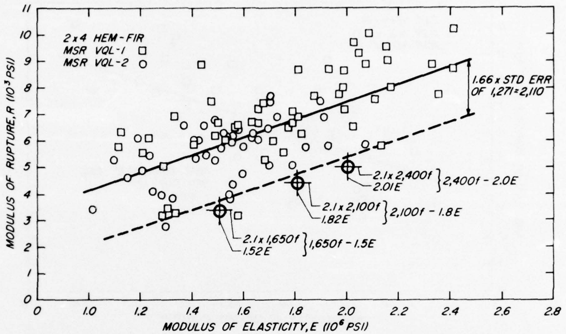
Figure 18.--Estimate of average E required to maintain F_b of grade.
