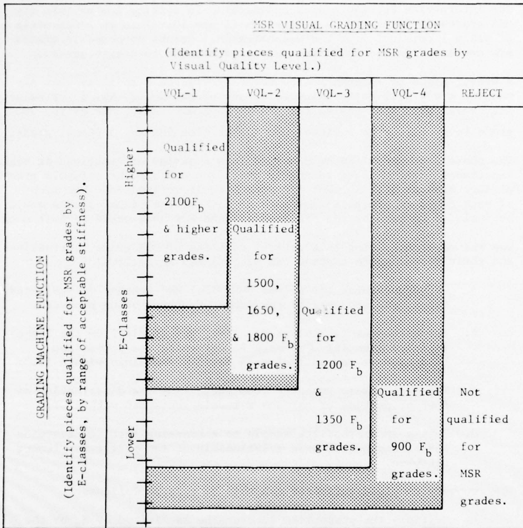
Figure 10.--Illustration of interaction of visual grading function (by grader) and the grading machine function (by machine) in sorting lumber by the MSR grade rules.
