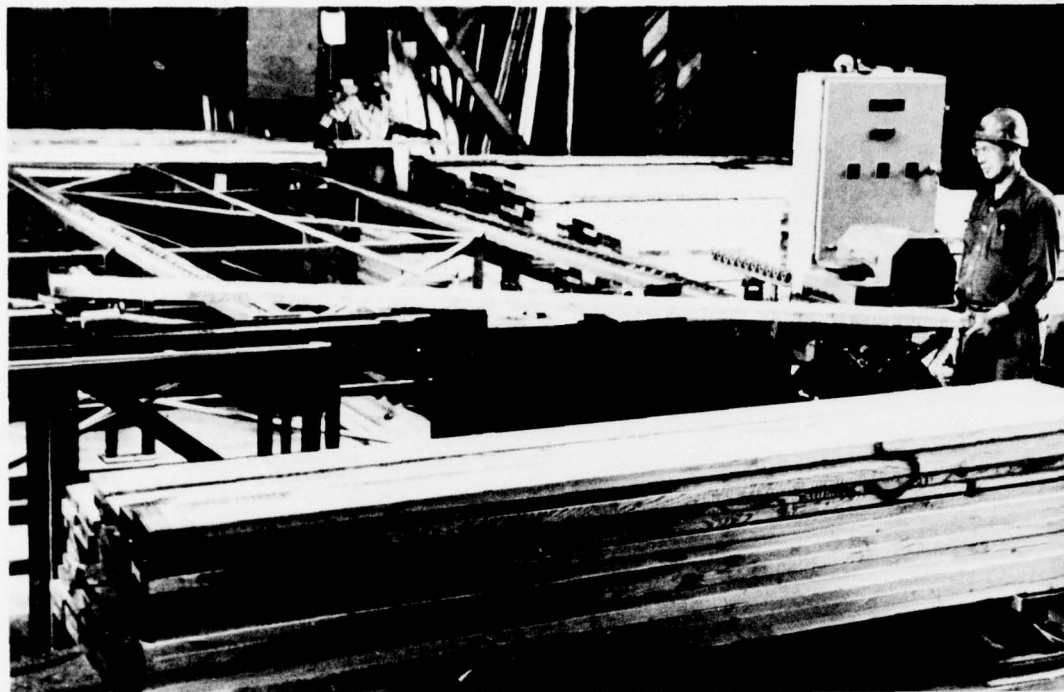
Figure 41.--Stress-Wave.
