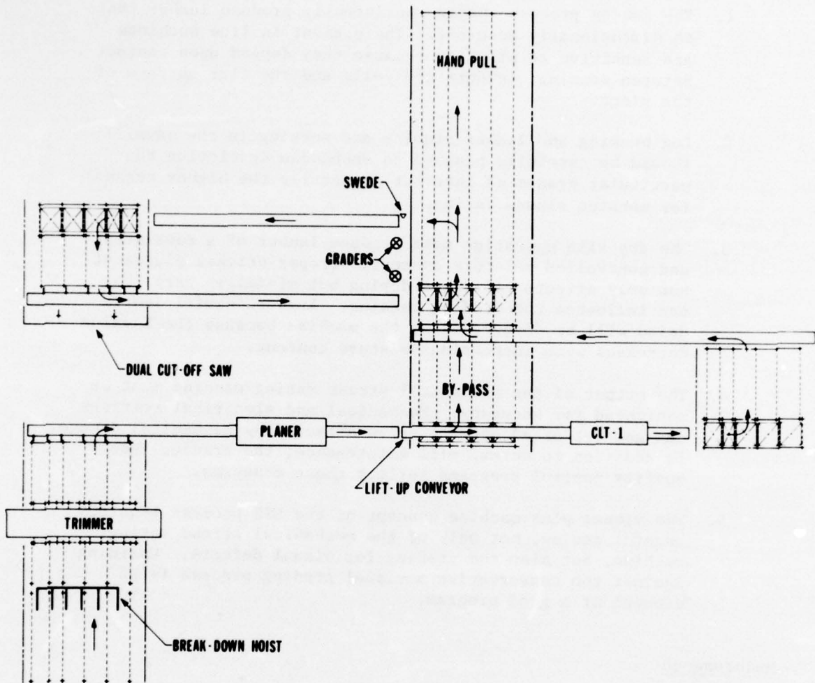
Figure 35.--A planing mill arrangement in which all lumber is trimmed prior to planing and in which all lumber is passed through the grading machine as the standard procedure. The by-pass permits mill operation with visual grading if the CLT-1 is out of operation.
