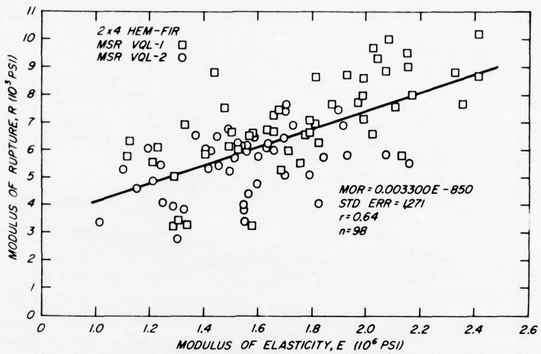
Figure 17.—Modulus of rupture (R) versus modulus of elasticity (E) flatwise, as measured with static tester.
