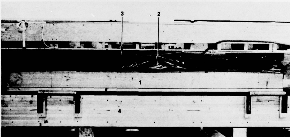
Figure 3 -- Distributed load set-up showing floor (1), air bag (2), strongback (3), and support (4). During test, floor was raised to reduce gap between the test specimen and the strongback. (M 139 508-12)
