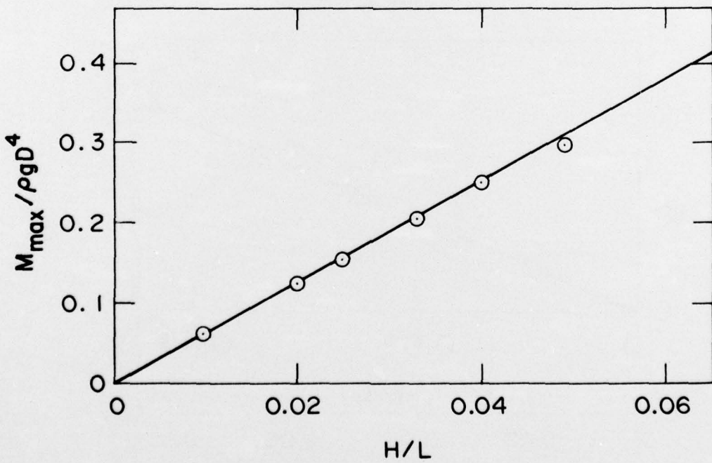
FIG. 14: MAXIMUM FORCES AND MOMENTS ( D/L = 0.128, d/L = 0.246 )
