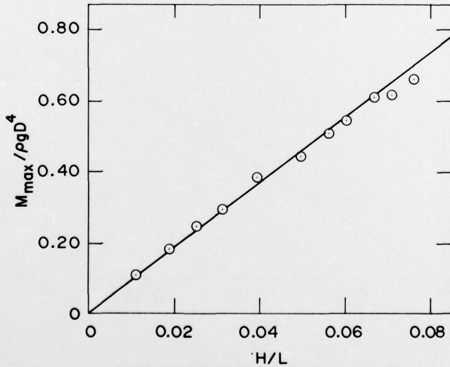
FIG. 15: MAXIMUM FORCES AND MOMENTS ( D/L = 0.123, d/L = 0.297 )
