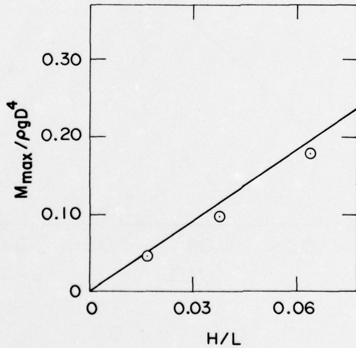
FIG. 10: MAXIMUM FORCES AND MOMENTS ( D/L = 0.325, d/L = 0.786 )
