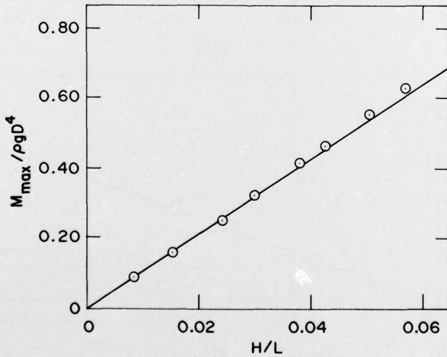
FIG. 18: MAXIMUM FORCES AND MOMENTS ( D/L = 0.092, d/L = 0.222 )
