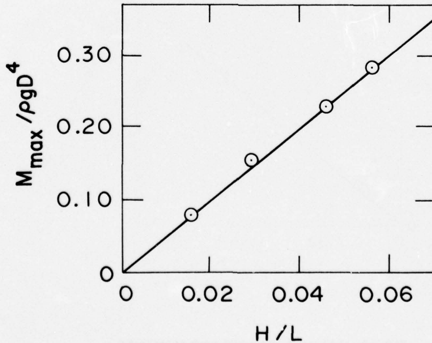
FIG. 11: MAXIMUM FORCES AND MOMENTS ( D/L = 0.239 , d/L = 0.578 )
