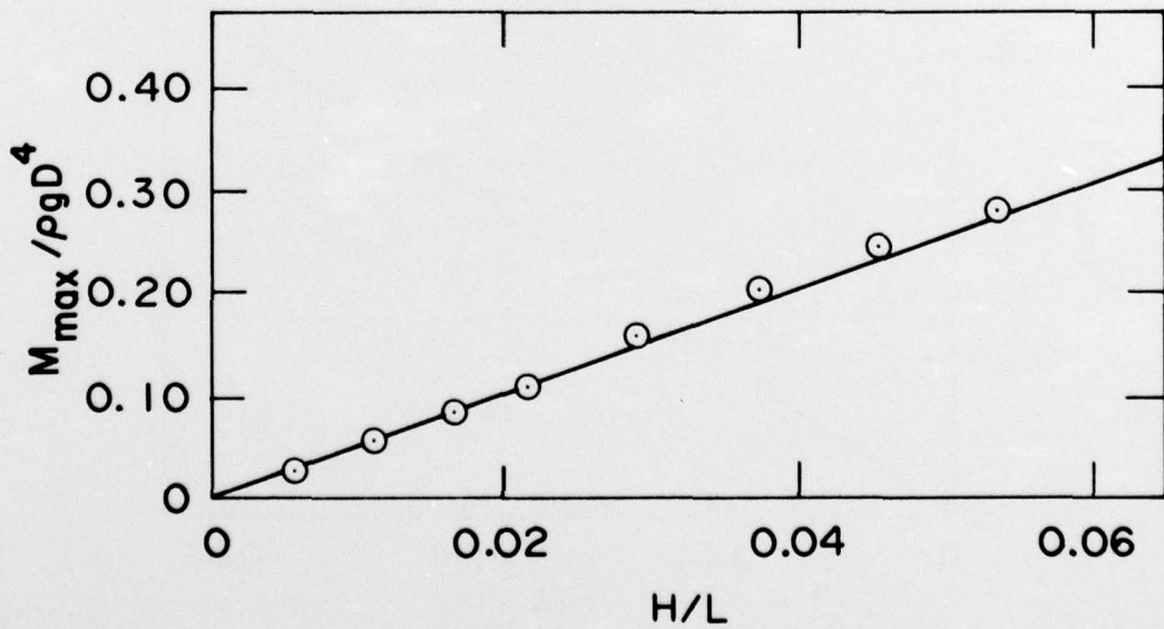
FIG. 17: MAXIMUM FORCES AND MOMENTS ( D/L = 0.105, d/L = 0.165 )
