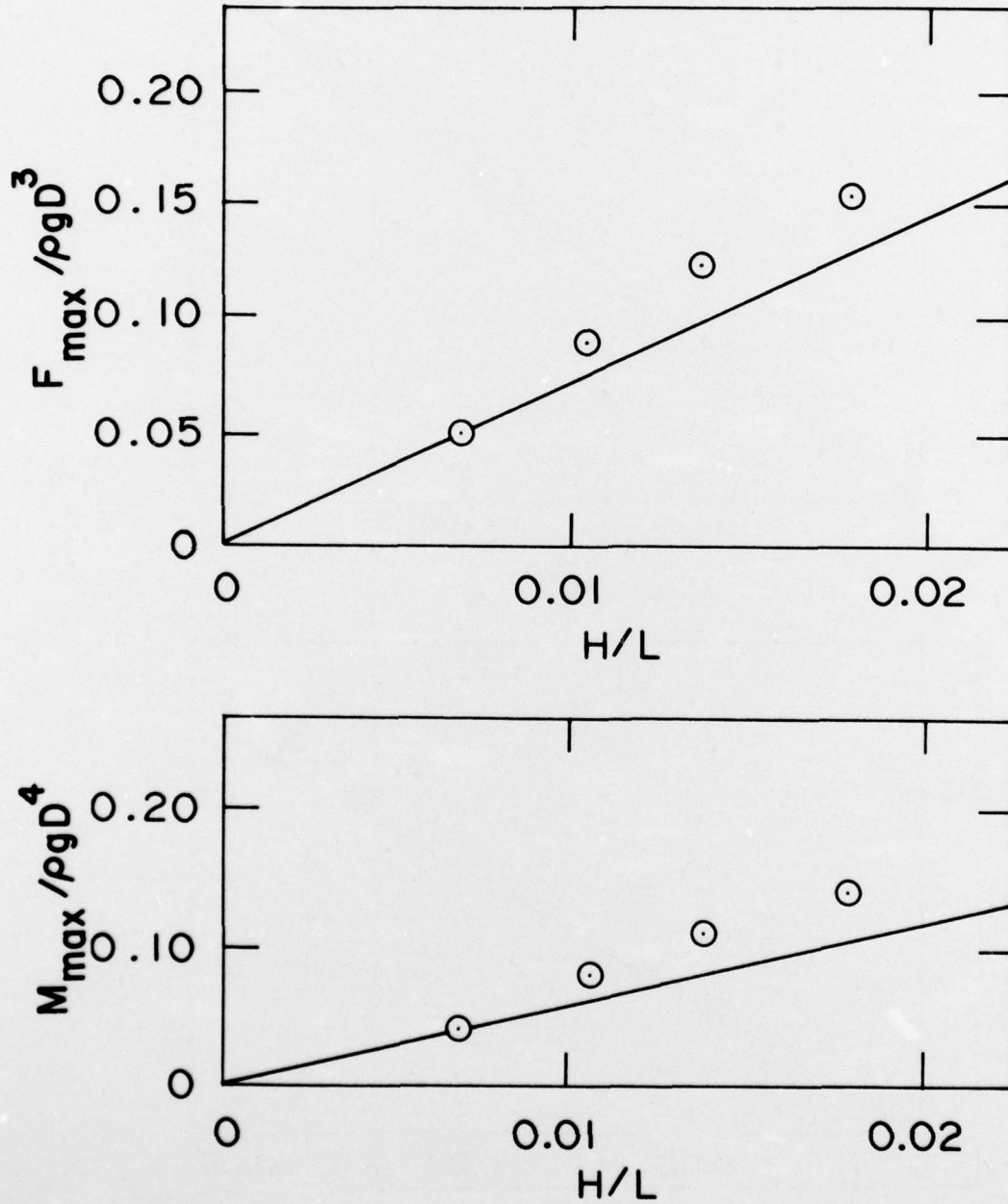
FIG. 22: MAXIMUM FORCES AND MOMENTS ( D/L = 0.057, d/L = 0.090 )
