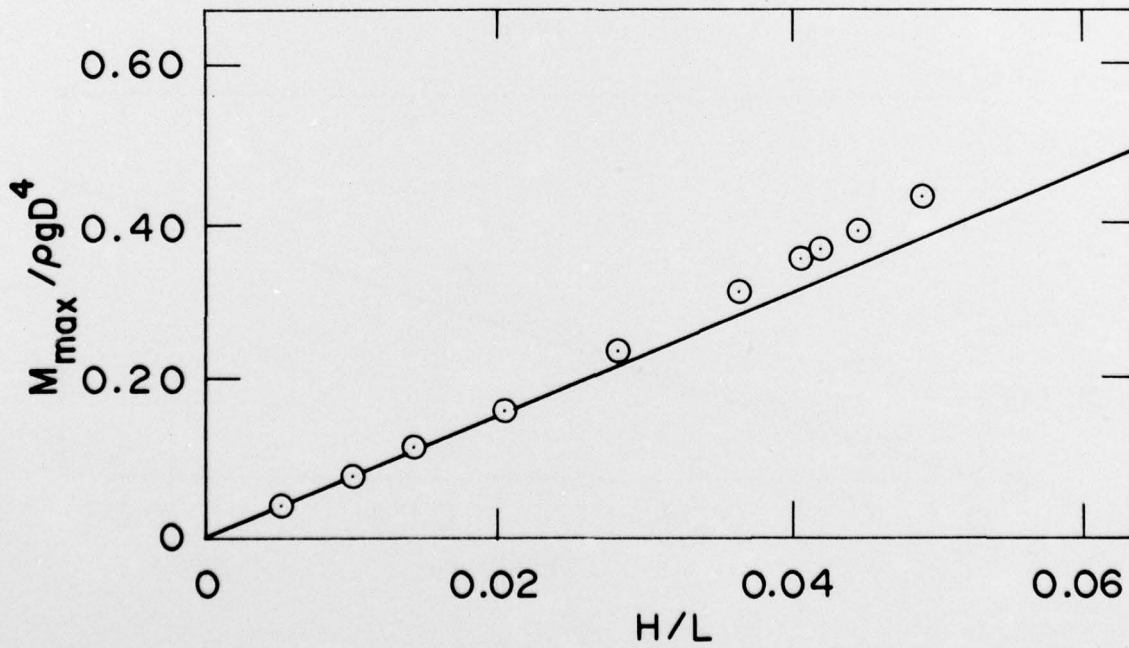
FIG. 20: MAXIMUM FORCES AND MOMENTS ( D/L = 0.080, d/L = 0.153 )
