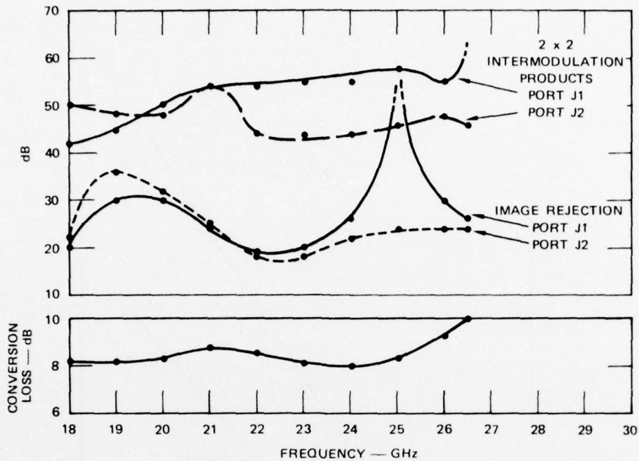
FIGURE II-5 CONVERSION LOSS, IMAGE REJECTION, AND 2 X 2 INTERMODULATION PRODUCTS FOR THE K-BAND (18.0 to 26.5 GHz), MIC, IMAGE-REJECT MIXER, MODEL KIRM-2(2). IF frequency = 168 MHz, diode bias currents = 1.0 mA, LO power input = 3.0 dBm.
