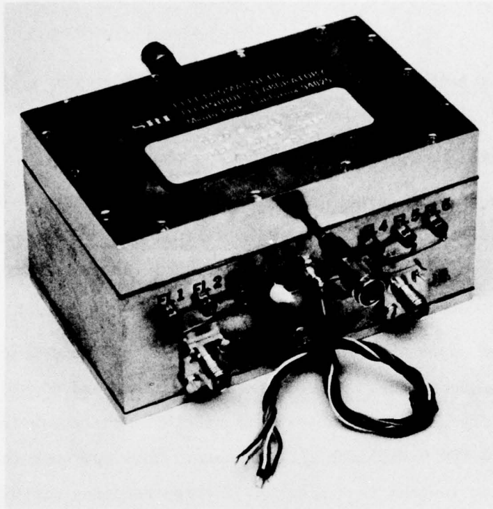
FIGURE II-1 K-BAND (18.0 to 26.5 GHz), MIC, IMAGE-REJECT MIXER, MODEL KIRM-2(2)
