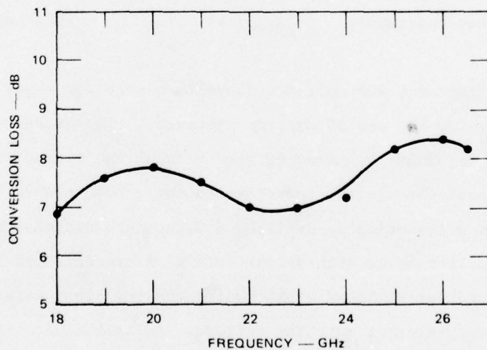
FIGURE II-11 CONVERSION LOSS FOR THE K-BAND (18.0 to 26.5 GHz), MIC, BALANCED MIXER, MODEL KDMIX-1. Diode bias currents = 1.0 mA, LO input power = 0 dBm.
