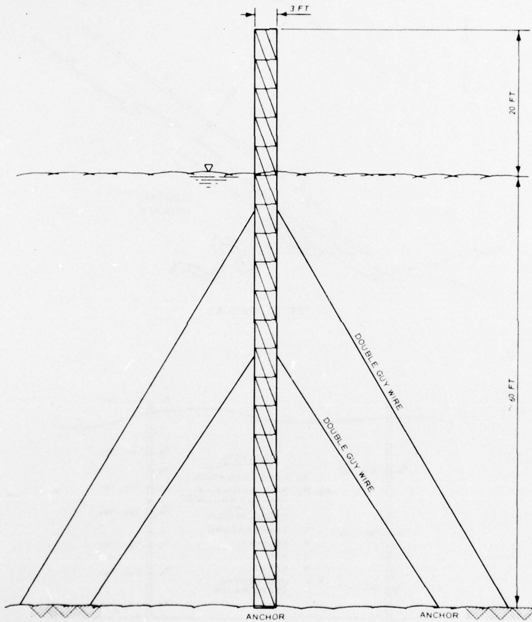
Figure 32. Schematic of instrumentation towers
