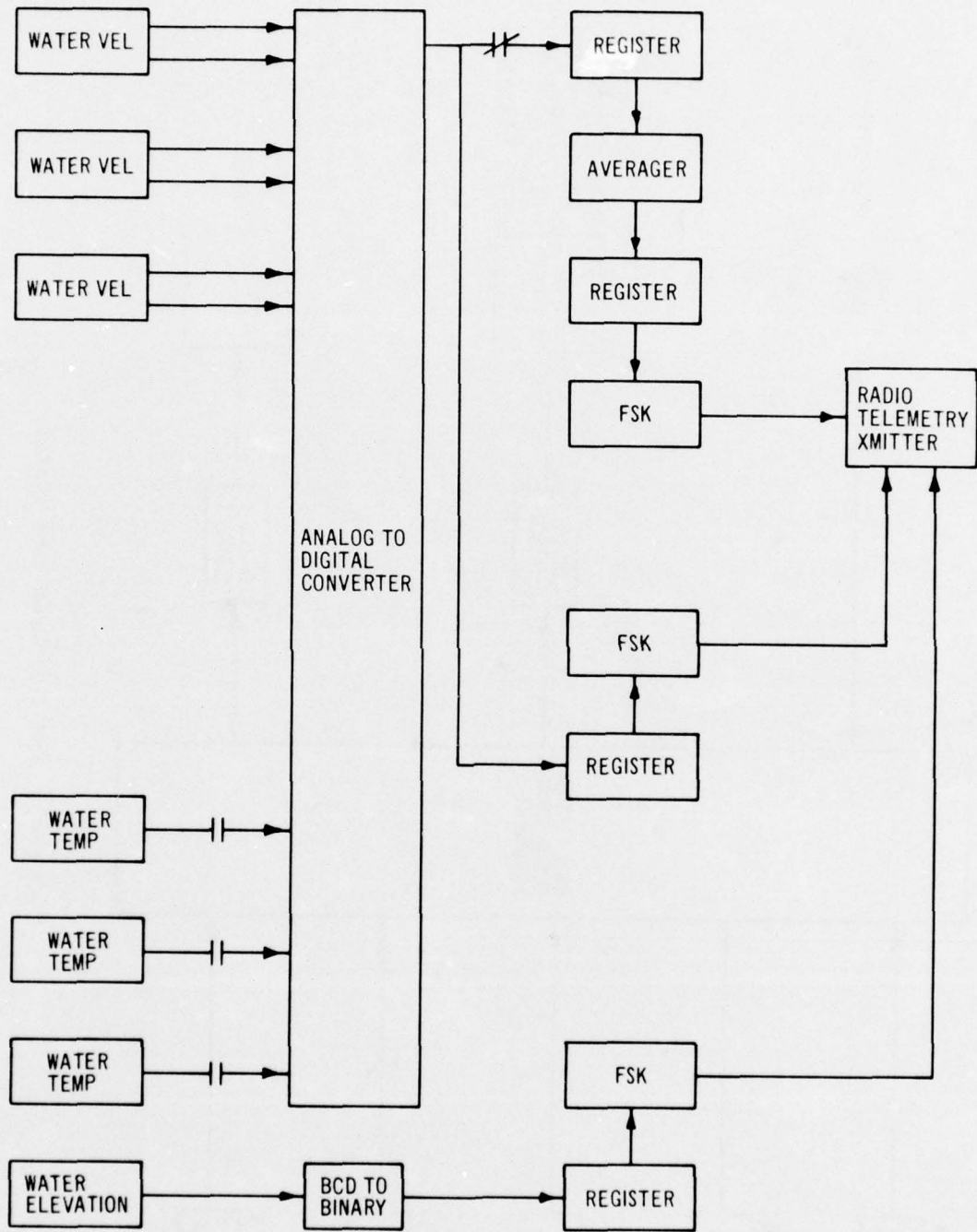
Figure 34. Block diagram locations A, C, and D
