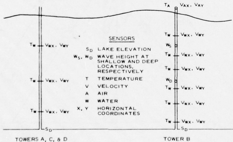
b. INSTRUMENTATION LOCATIONS
