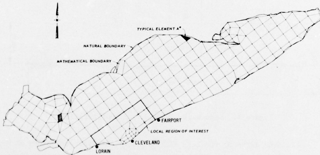
Figure 3. Finite element representation of Lake Erie
