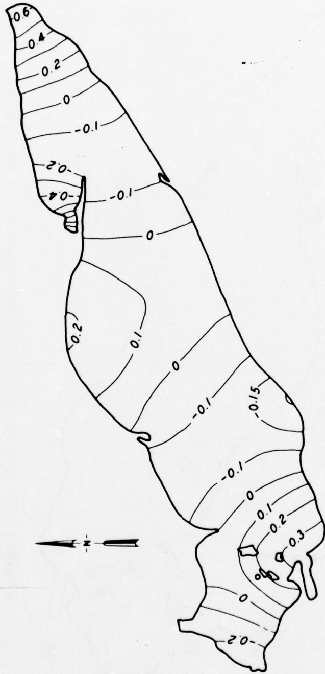
Figure 15. Mode shape of the fifth eigenvalue for the full lake without jetport (normalized to maximum elevation 1)
