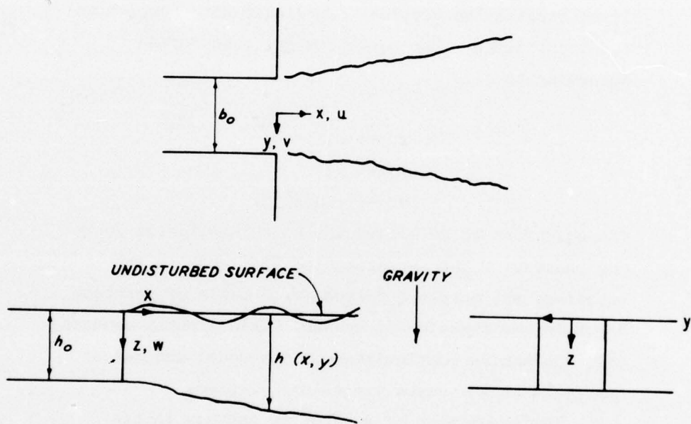
Figure 28. Geometry for three-dimensional jet
