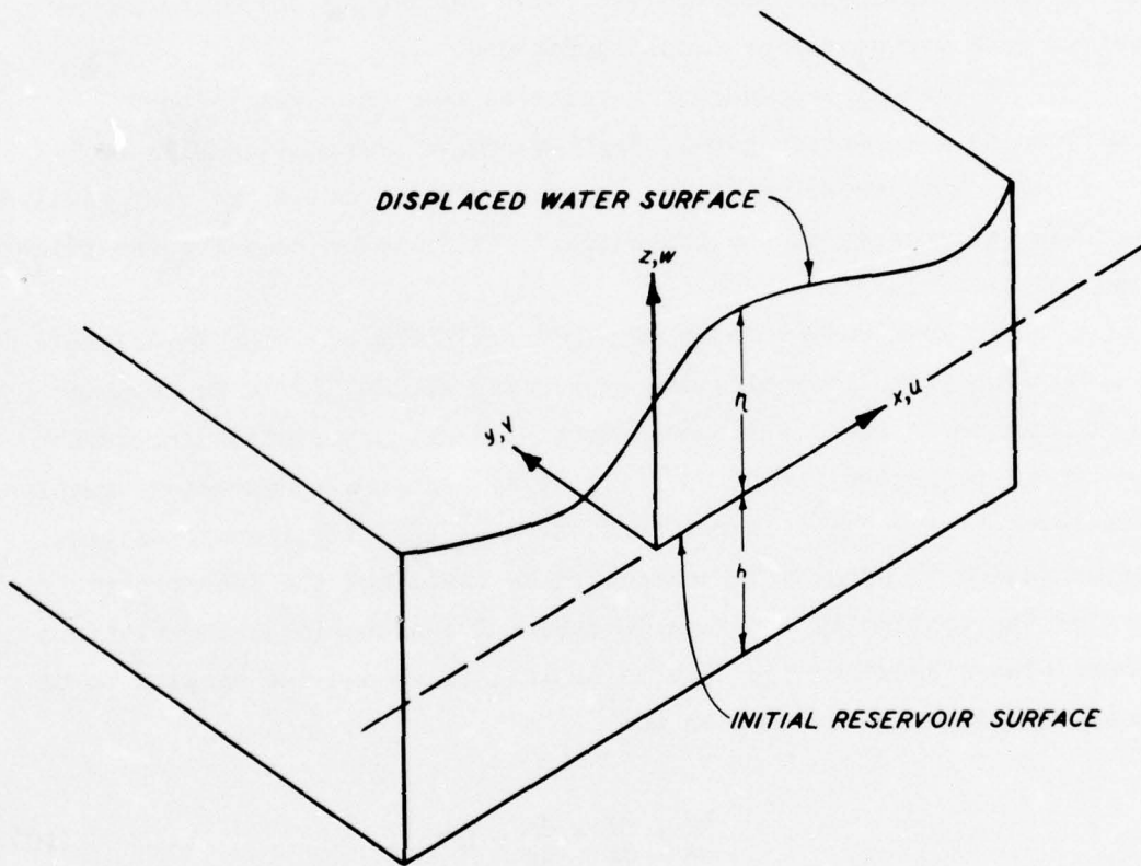
Figure 23. Coordinate system for problem formulation
