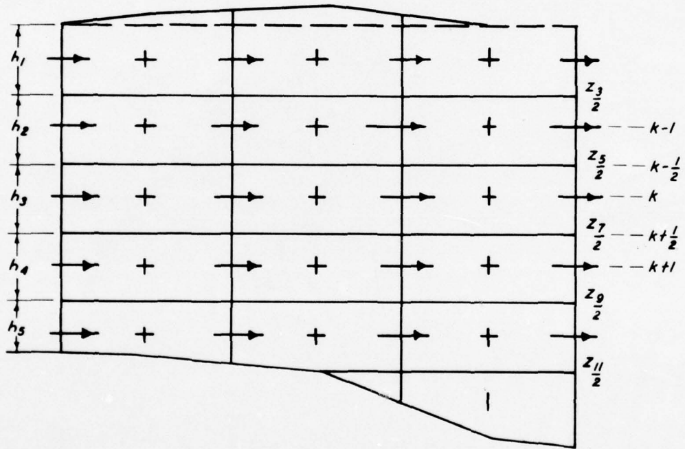
Figure 25. Location of variables of the vertical grid
