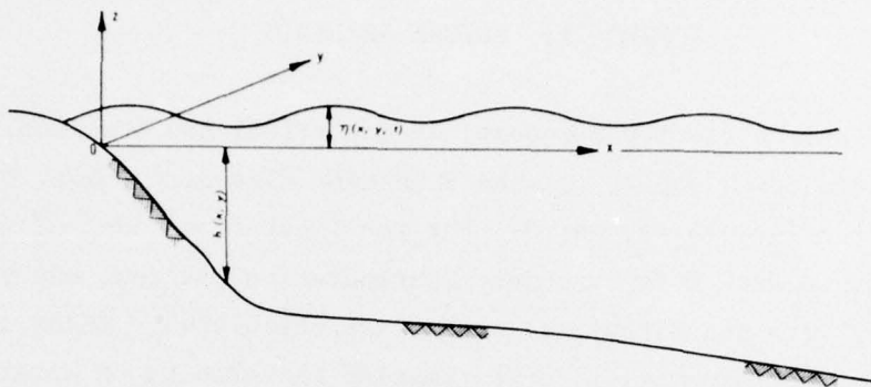
Figure 1. Coordinate system and surface profile
