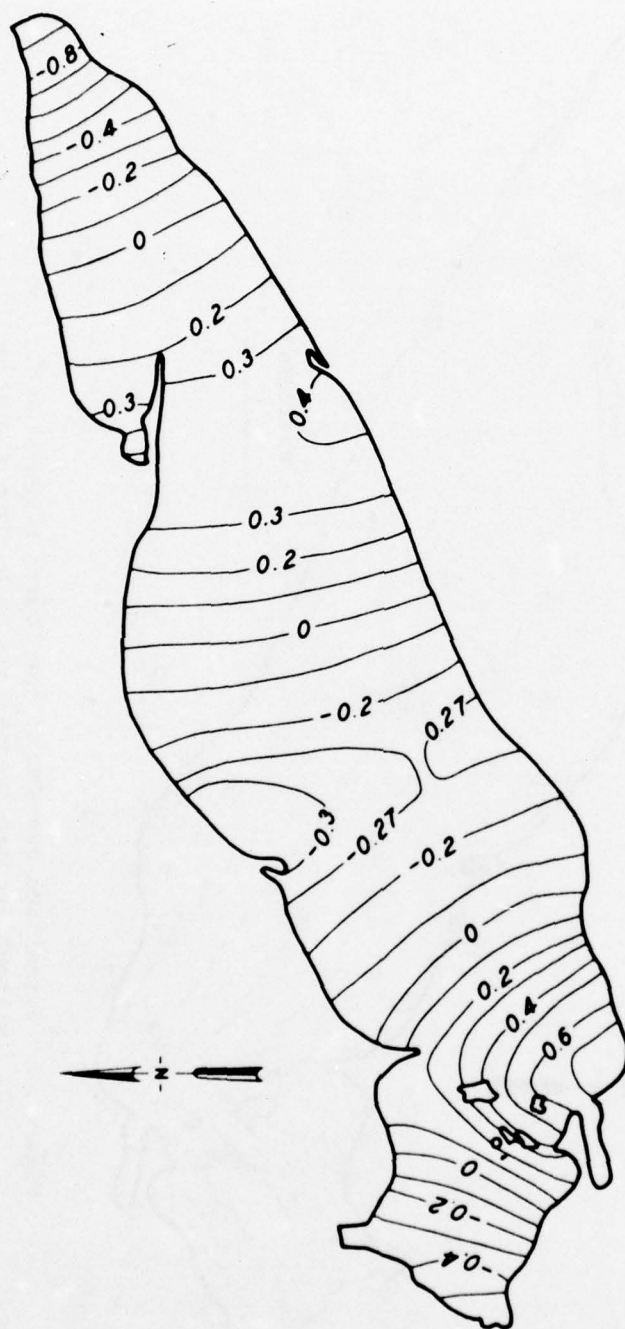
Figure 13. Mode shape of the fourth eigenvalue for the full lake without jetport (normalized to maximum elevation 1)
