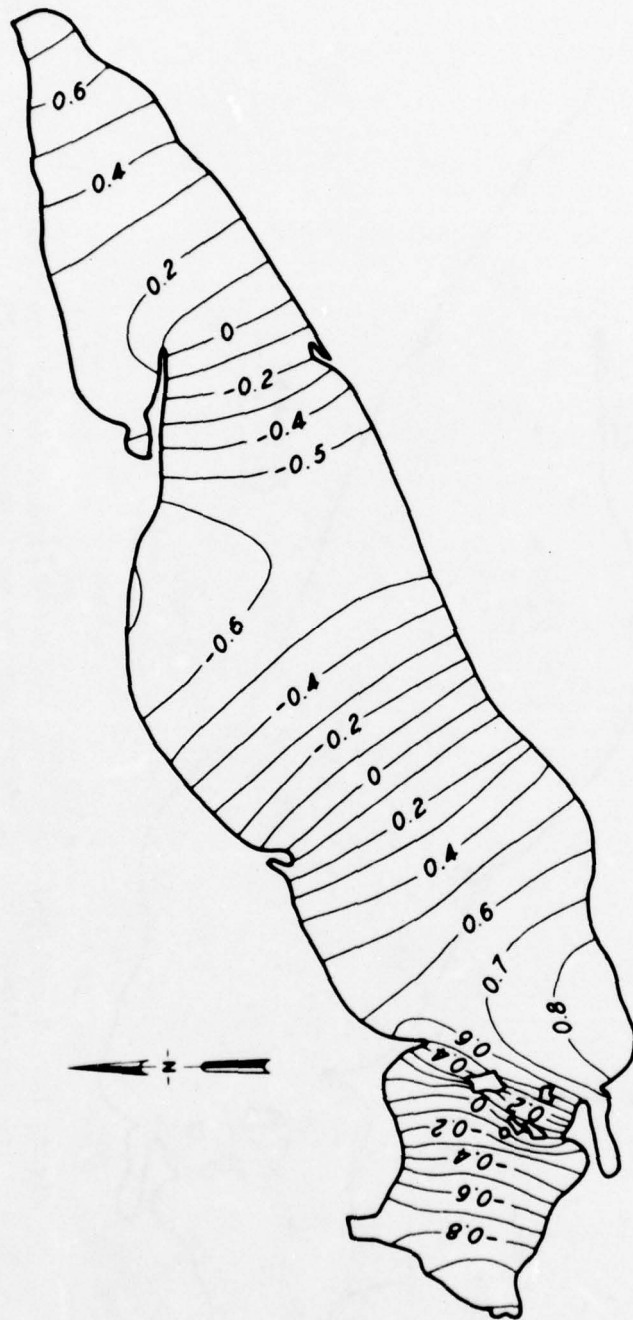
Figure 11. Mode shape of the third eigenvalue for the full lake without jetport (normalized to maximum elevation 1)
