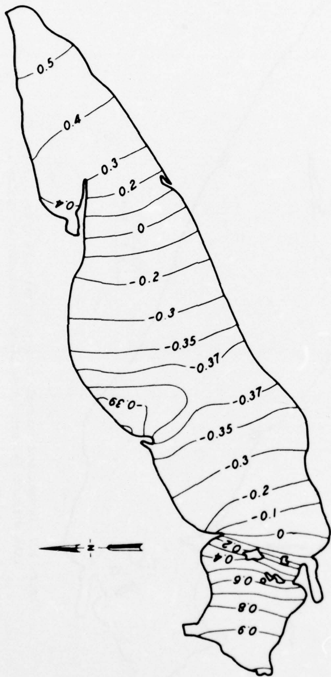
Figure 9. Mode shape of the second eigenvalue for the full lake without jetport (normalized to maximum elevation 1)
