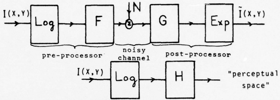
Fig. 5.7- Rom's result for transmission of an achromatic image over a noisy channel when the error criterion is a square error in the "perceptual" space.
