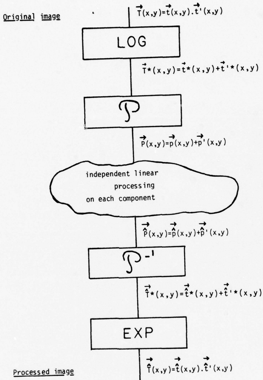
Fig. 4.8- Homomorphic interpretation when linear processing is performed in the "perceptual" space. Notice at every step the harmony between the processing and the structure of the processed quantities.
