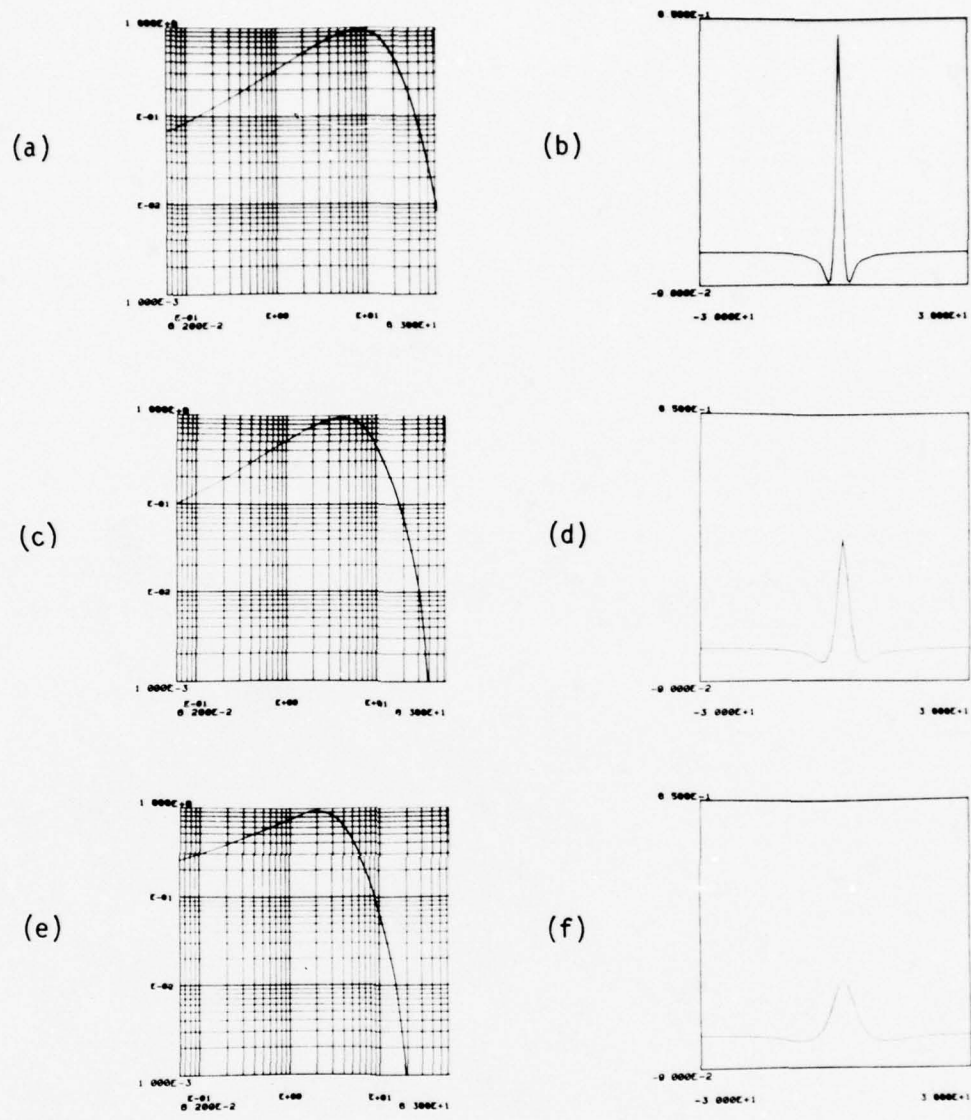
Fig. 3.9- The frequency responses H(f) , H_1(f) and H_2(f) of the filters operating on the A, C_1 and C_2 signals (a, c, e), respectively, and (b, d, f) the corresponding point-spread functions h(x) , h_1(x) and h_2(x) . The frequency responses are plotted on a log-log scale, the point-spread functions for a span of one degree of visual angle.
