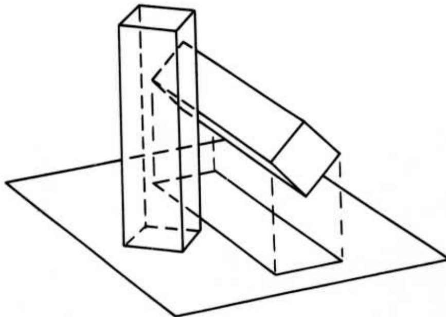
Figure 8 Separating plane not a polyhedron face
