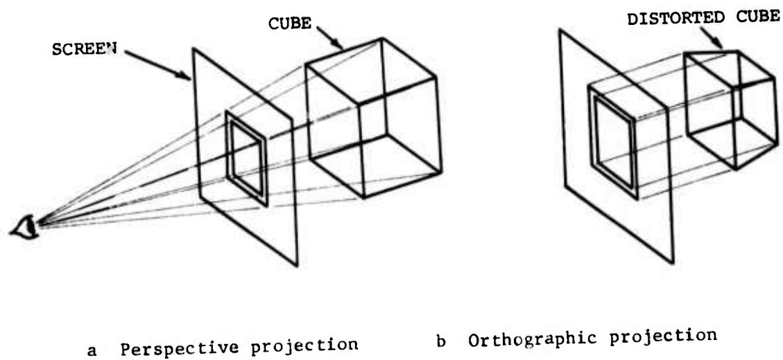
Figure 1 Distortion of cube by perspective transformation
