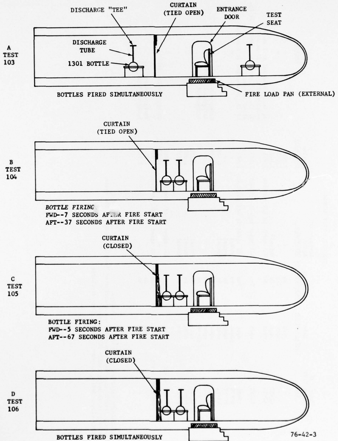
FIGURE 3. PRELIMINARY TEST HALON 1301 DISCHARGE LOCATIONS
