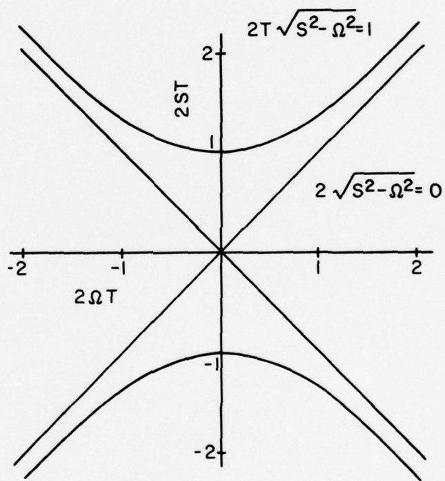
Figure 4. The Criterion for Molecular Expansion in a Two-Dimensional Flow (Lumley, 1972).
