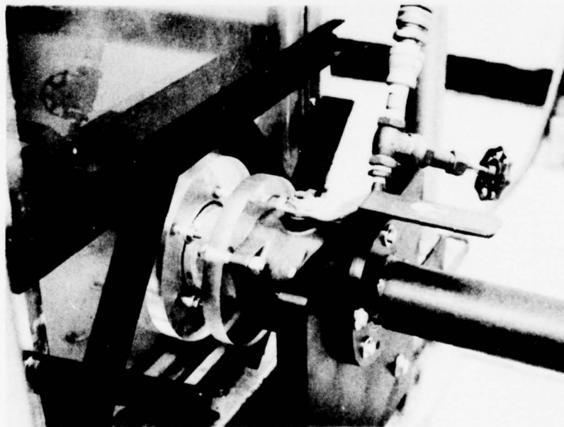
Figure 14. Photograph of the Smooth Entrance Piece Connected Between the Test Tank and the Ball Valve (Handle in the Open Position).
