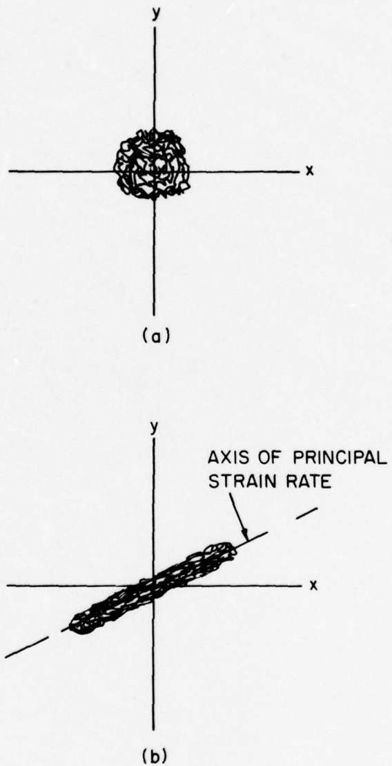
Figure 3. Sketches of the Unstrained (a) and Strained (b) State of the Polymer Molecules in Solution.
