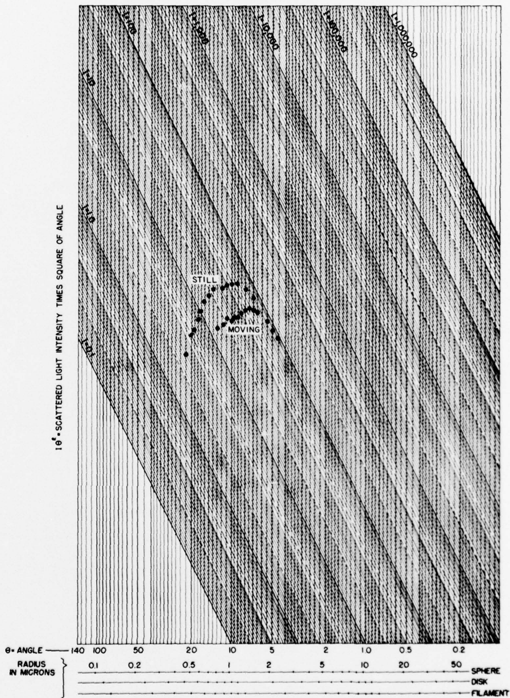
Figure 27. Scattered Light Intensity Times the Square of the Angle of Scatter Versus Angle of Scatter. Velocity = 19.2 fps., Concentration = 1600 ppmw., Position = 0.85.
