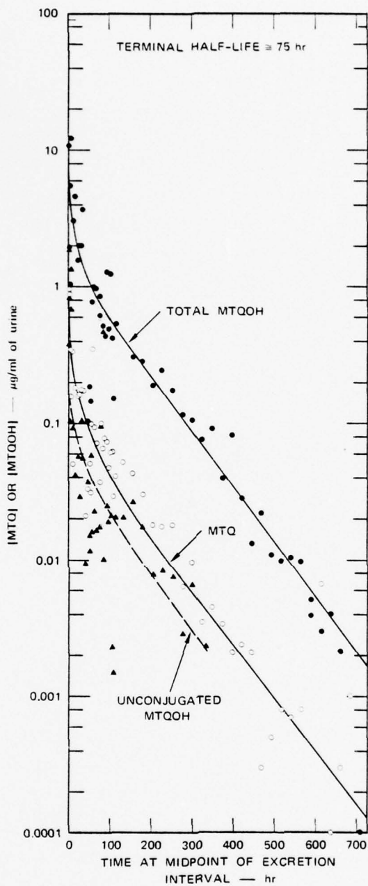
FIGURE 9 CONCENTRATIONS OF METHAQUALONE, TOTAL 6-HYDROXYMETHAQUALONE, AND UNCONJUGATED 6-HYDROXYMETHAQUALONE IN URINE VERSUS TIME AT MIDPOINT OF EXCRETION INTERVAL
