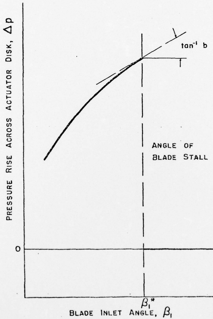
Figure 2. Pressure rise as a function of inlet angle.
