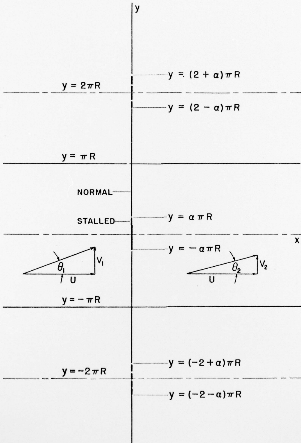
Figure 4. Pattern of stalled and unstalled regions on actuating line.
