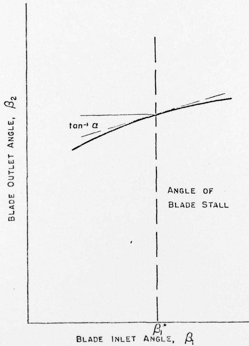
Figure 3. Discharge angle as a function of inlet angle.
