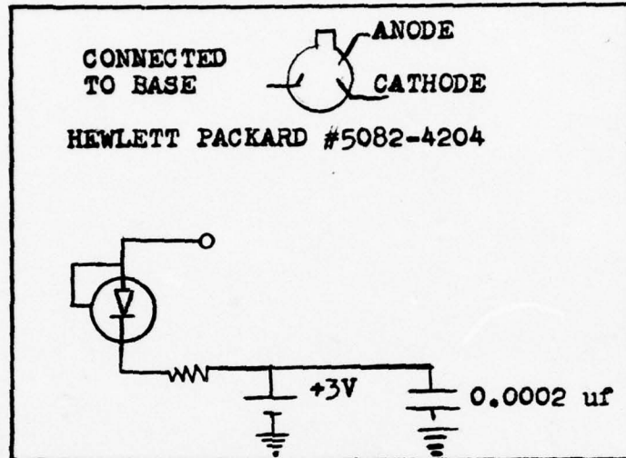
Fig. 4. Photo Detector.
