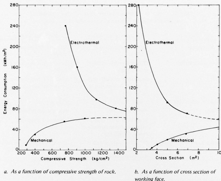
Figure 14. Energy consumption (per unit volume) for excavating material by mechanical cutting and by high-frequency electrothermal irradiation as a function of compressive strength of rock and cross section of working face.
