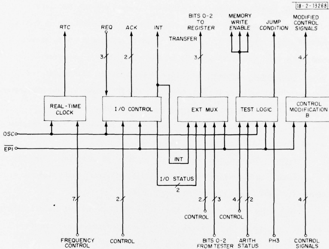
Fig. A3. The control B gate array.
