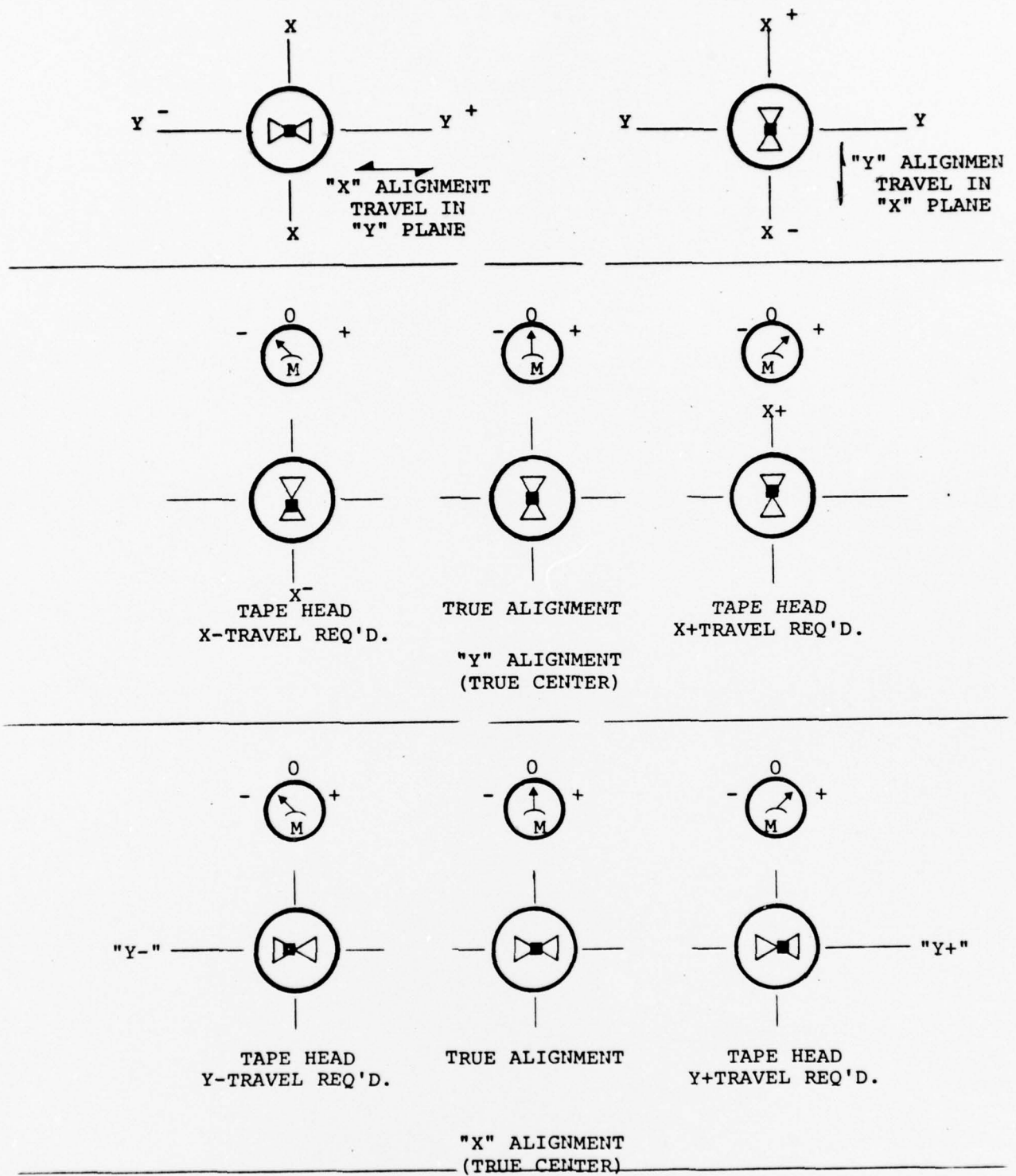
FIGURE 4-18 ILLUS BOW-TIE ALIGNMENT ORIENTATION
