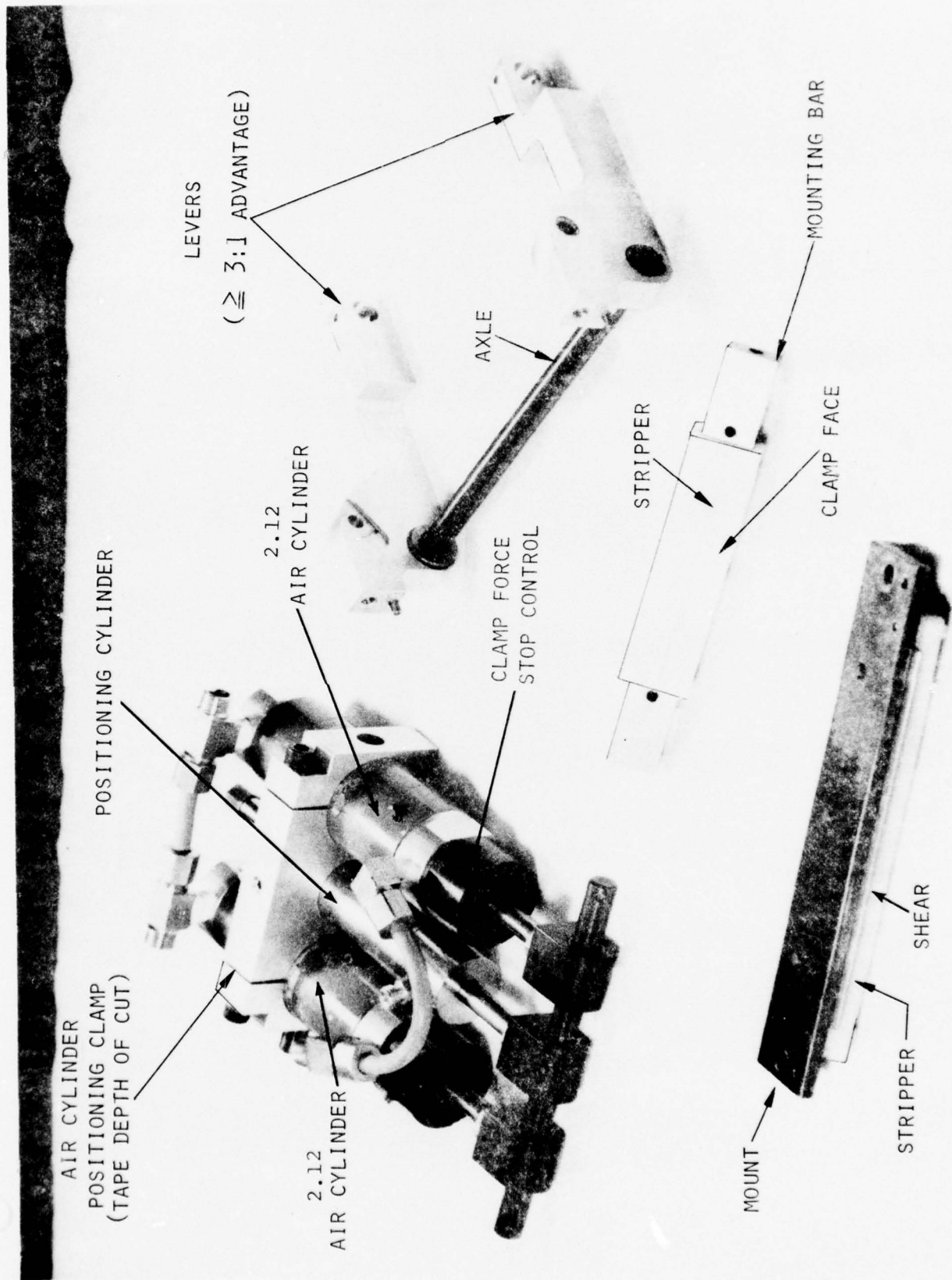
FIGURE 5-25 SHEAR/CLAMP, SUBASSY UNIV HOLDING
