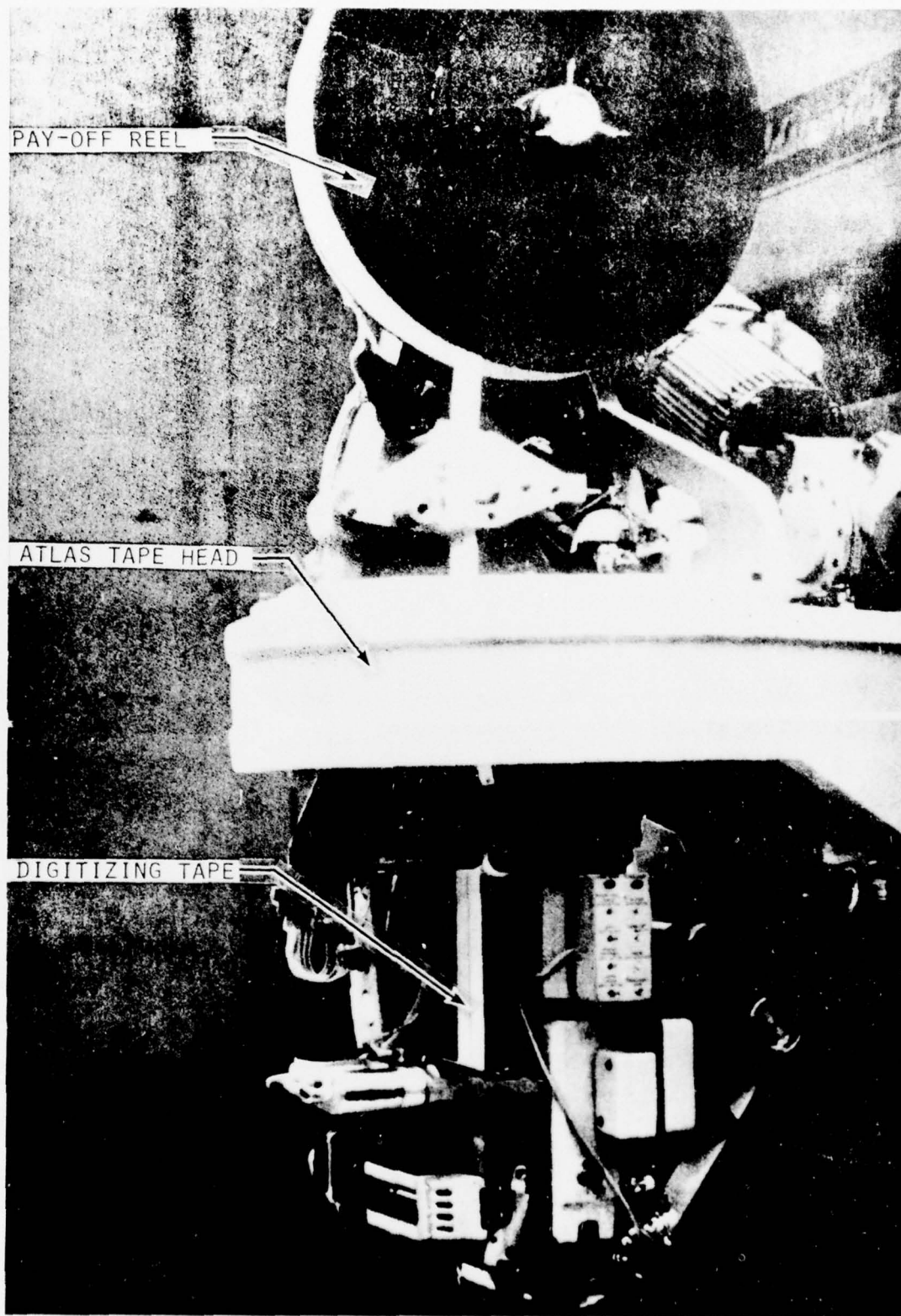
FIGURE 3-3 VIEW, DIGITIZING TAPE INSTALLED
