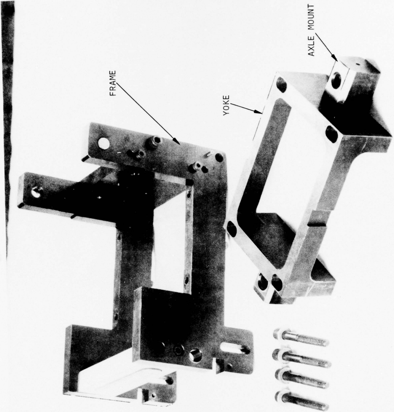
FIGURE 5-23 BASIC FRAME PARTS UNIVERSAL HOLDER
