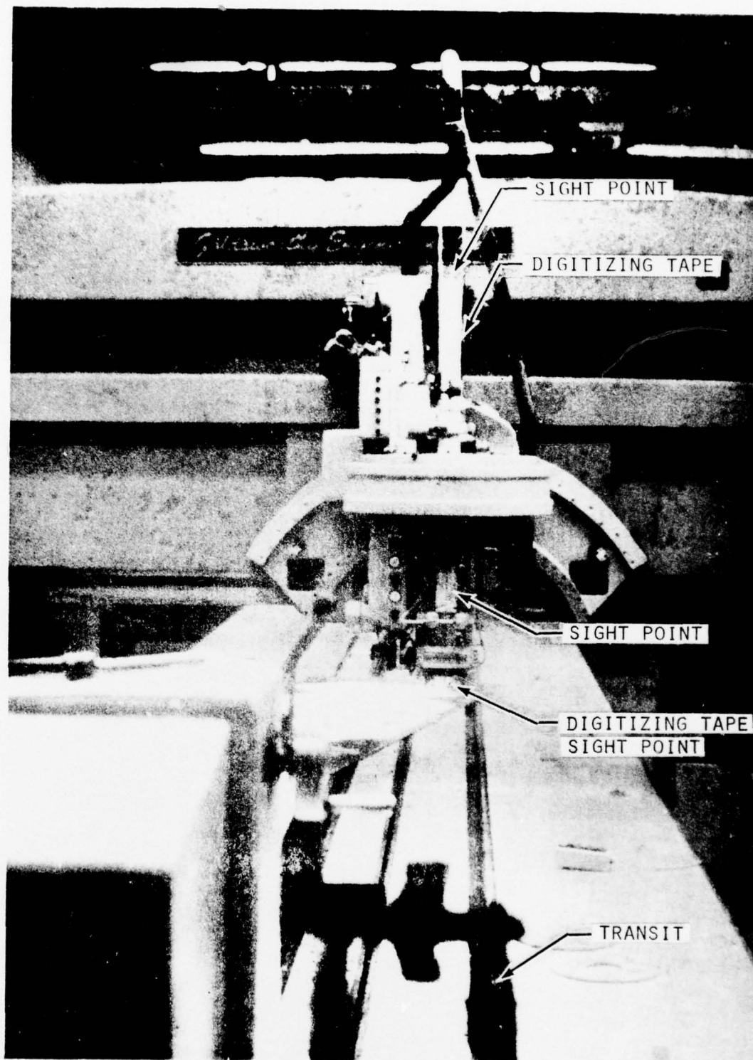
FIGURE 3-1 ATLAS MACH. ALIGN. SET-UP
