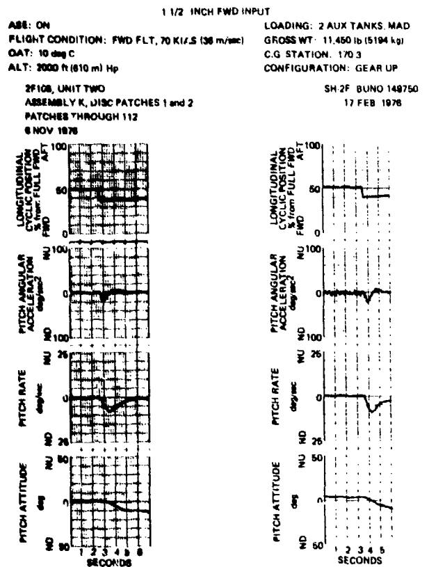
Figure 4 Pitch Axis Control Response
