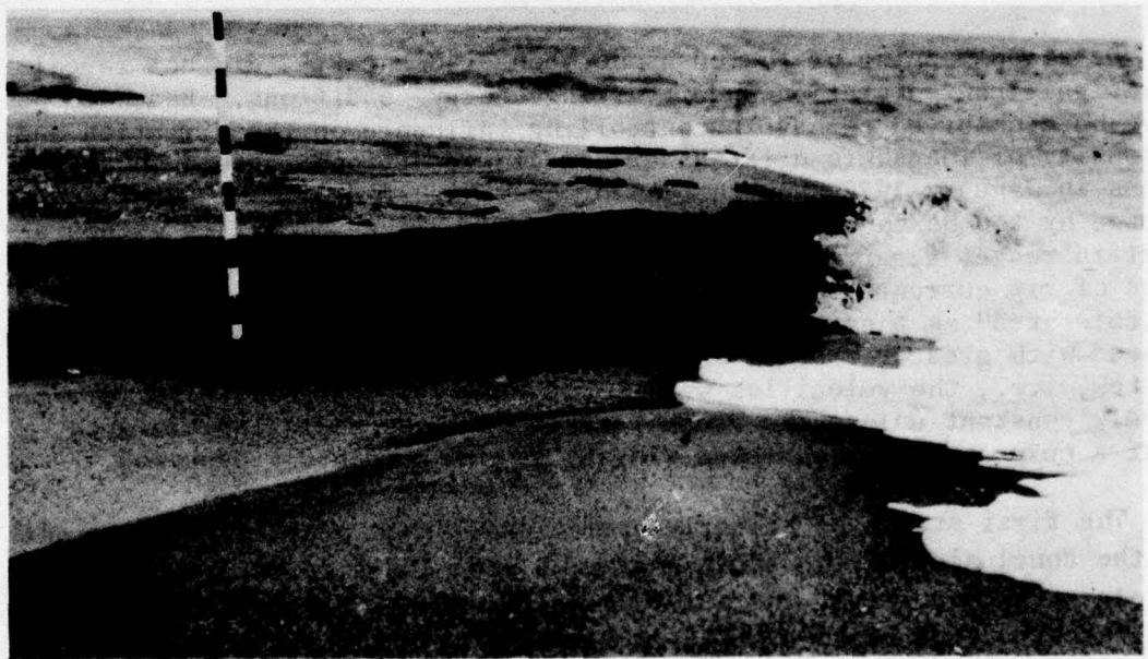
Figure 61. Frozen berm crest and beach face at high tide. Greater current velocities in cusp bays may erode through the ice cover.
