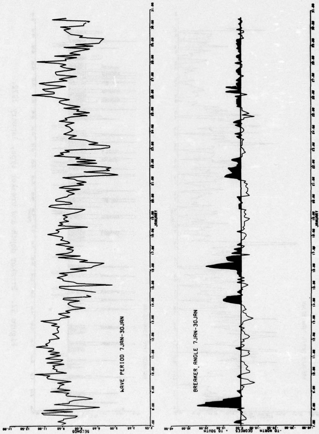
Figure 51. Wave period and breaker angle, January 1972.
