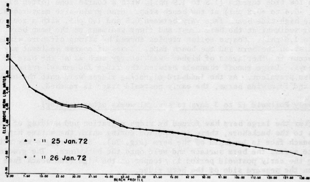
Figure 67. Profiles PL-7 and PL-11, 25 and 26 January 1972.
