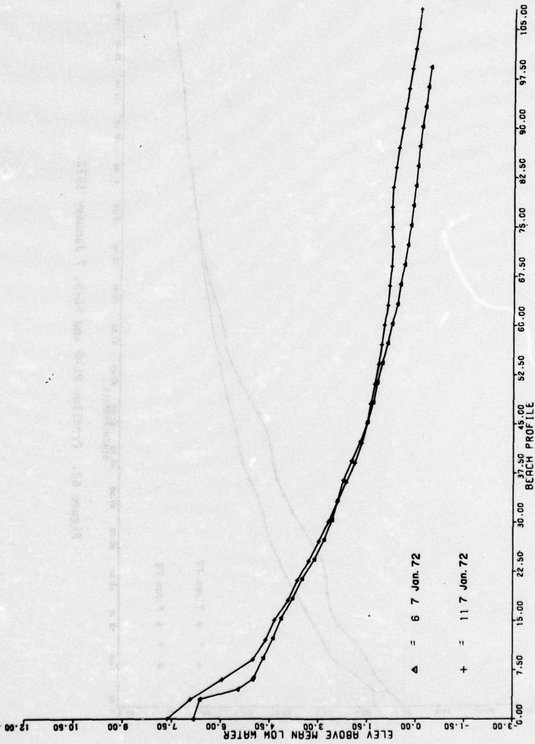
Figure 63. Profiles PL-6 and PL-11, 7 January 1972.
