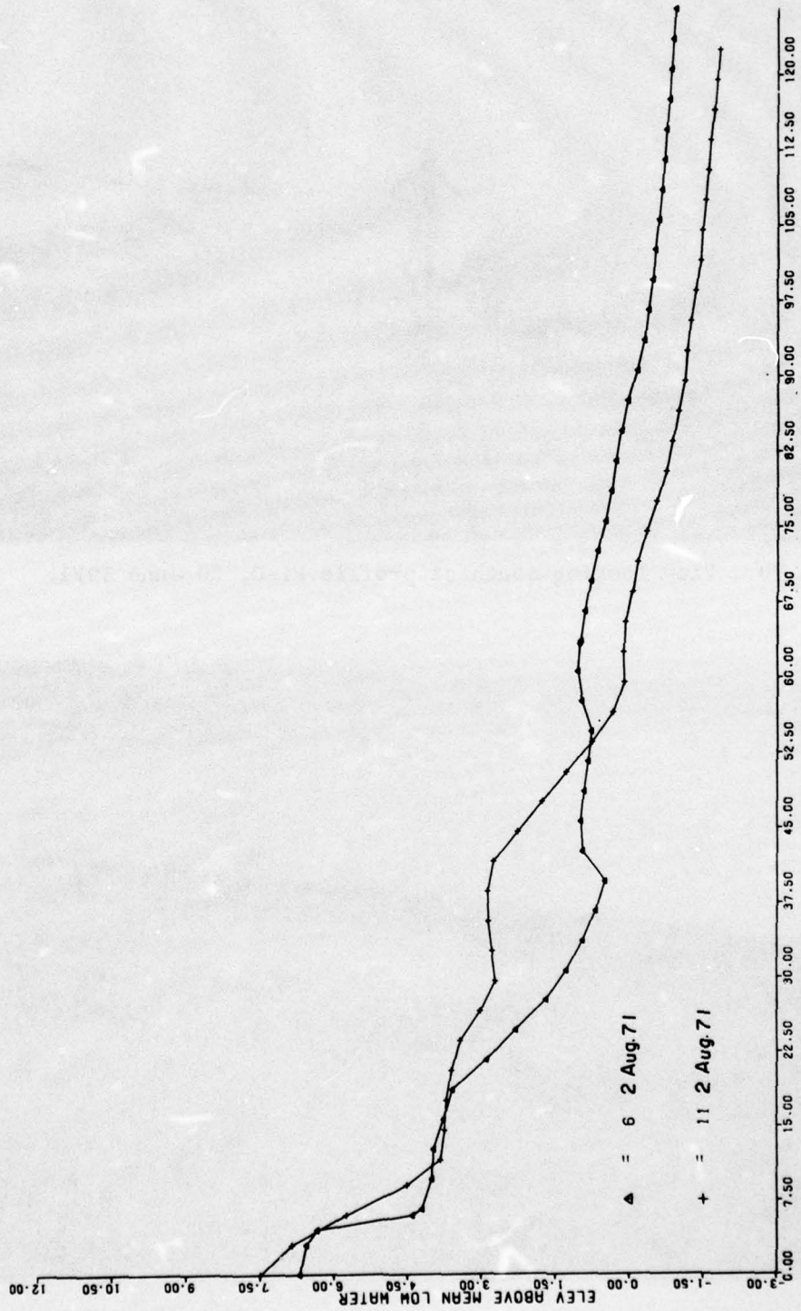
Figure 19. Profiles PL-6 and PL-11, 2 August 1971.
