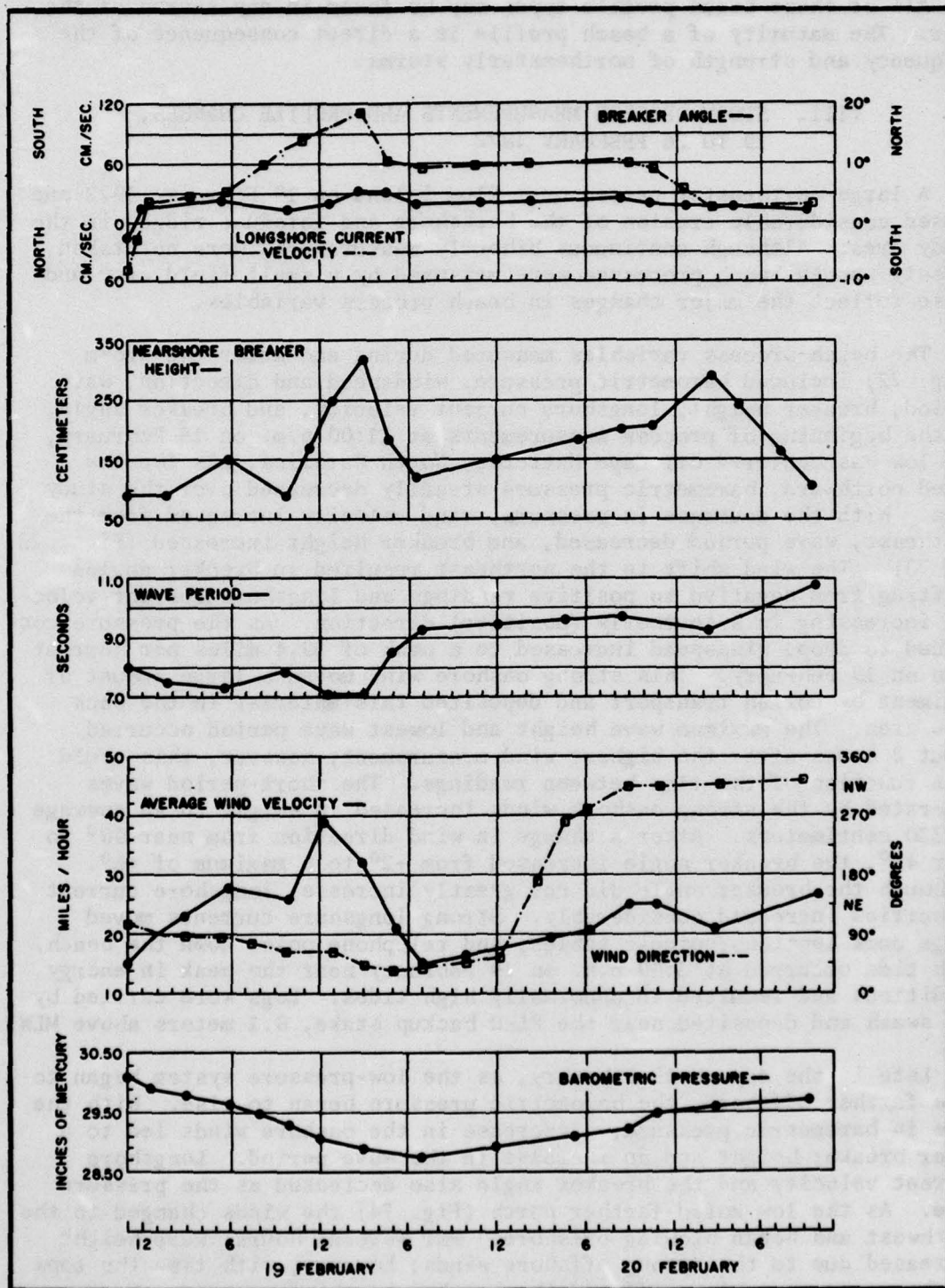
Figure 72. Beach process variable measurements, 18 to 20 February 1972.
