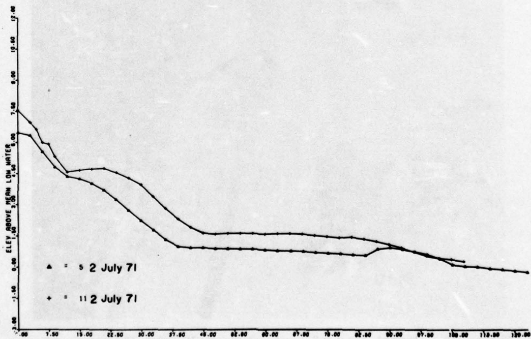
Figure 15. Profiles PL-5 and PL-11, 2 July 1971.
