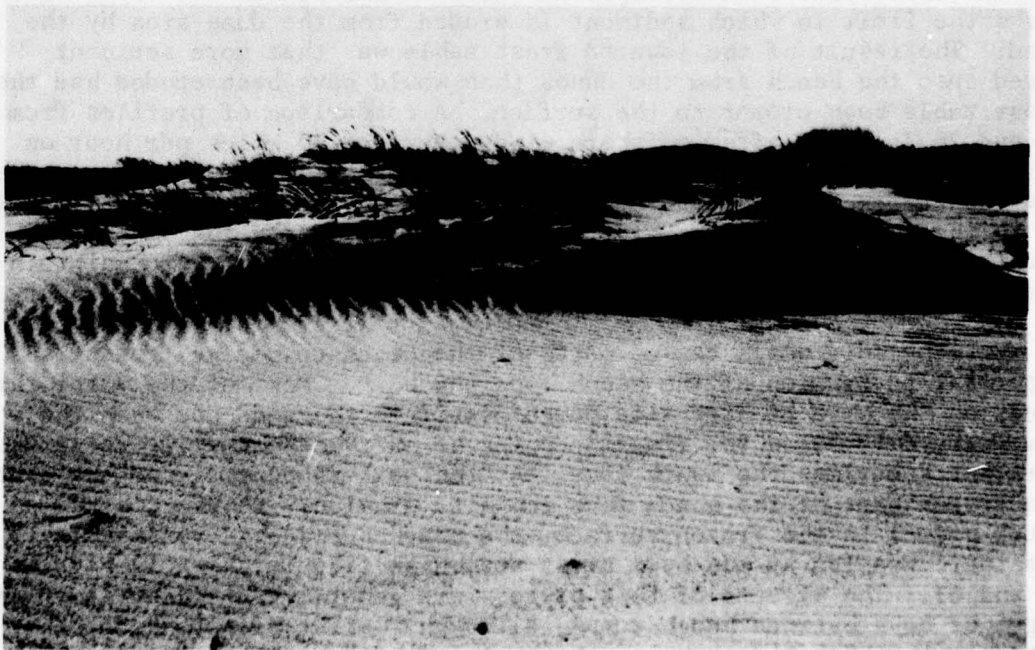
Figure 56. Poststorm beach, profile PL-0. Note eolian ripples in back dune area. View toward southwest.
