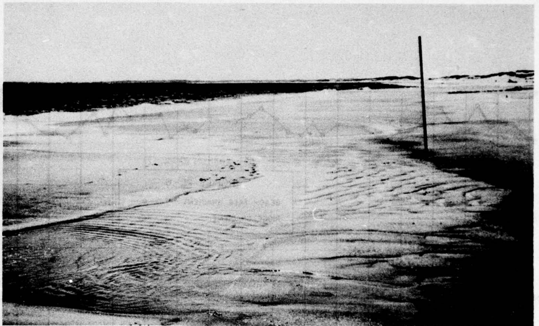
Figure 22. Initial swash overtopping ridge. Note small ridges. Scale is 3 meters.
