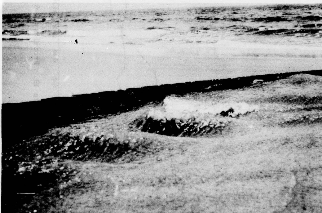
Figure 21. Upper flow regime conditions in a runoff channel, which has dissected the ridge surface near PL-0.
