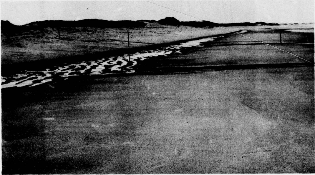
Figure 34. Photo of profile PL-0 looking north, 22 July 1971.
