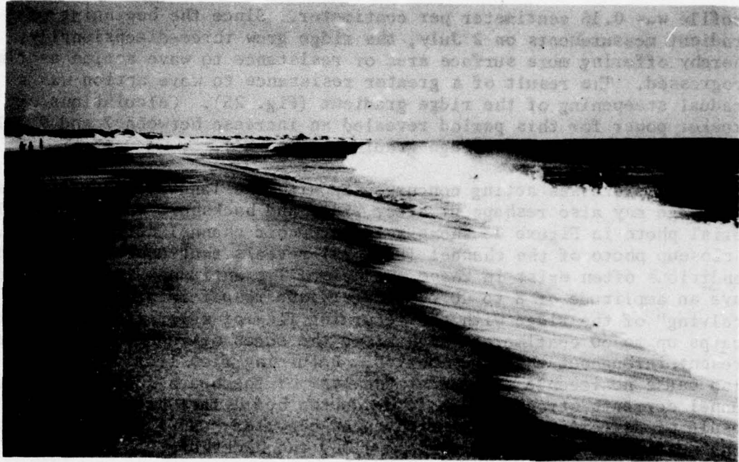
Figure 25. Wave steepening of ridge gradient.
