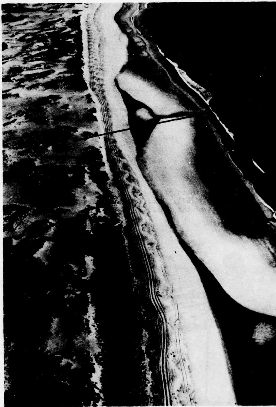
Figure 40. Aerial view of northern half of study area, 25 July 1971 (profile PL-7).
