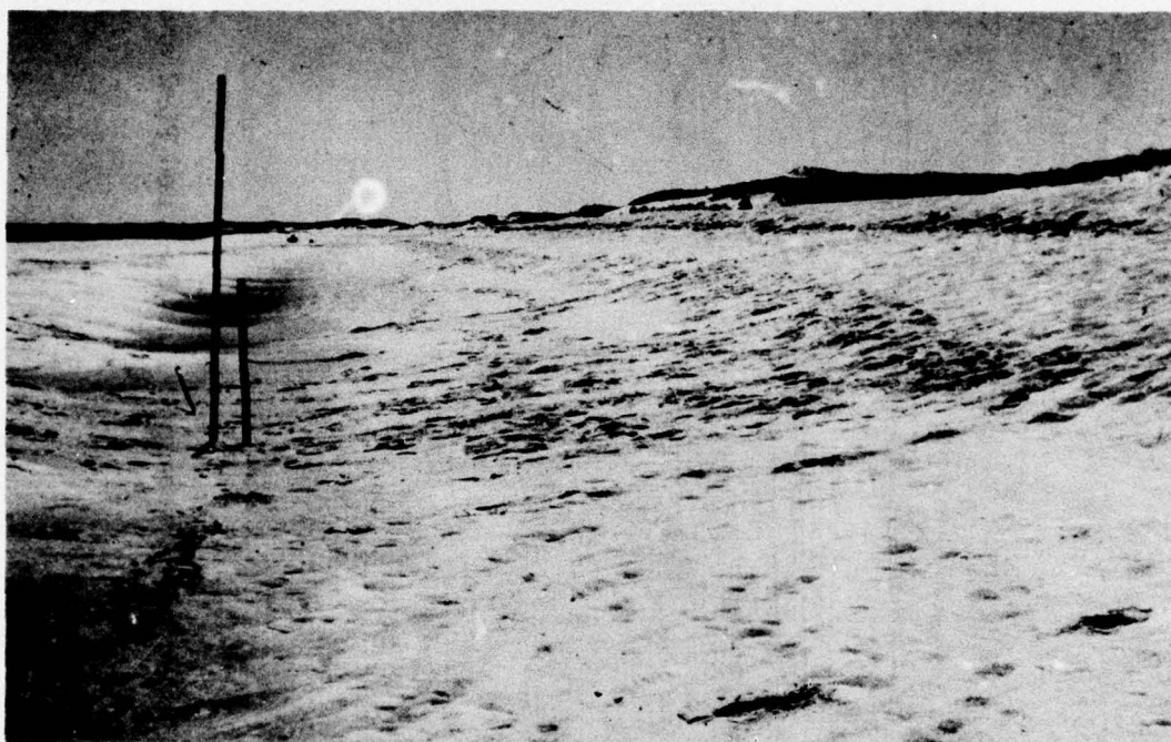
Figure 30. Profile PL-0 on 12 July 1971, looking south. Note berm runnel. Scale is 300 centimeters.
