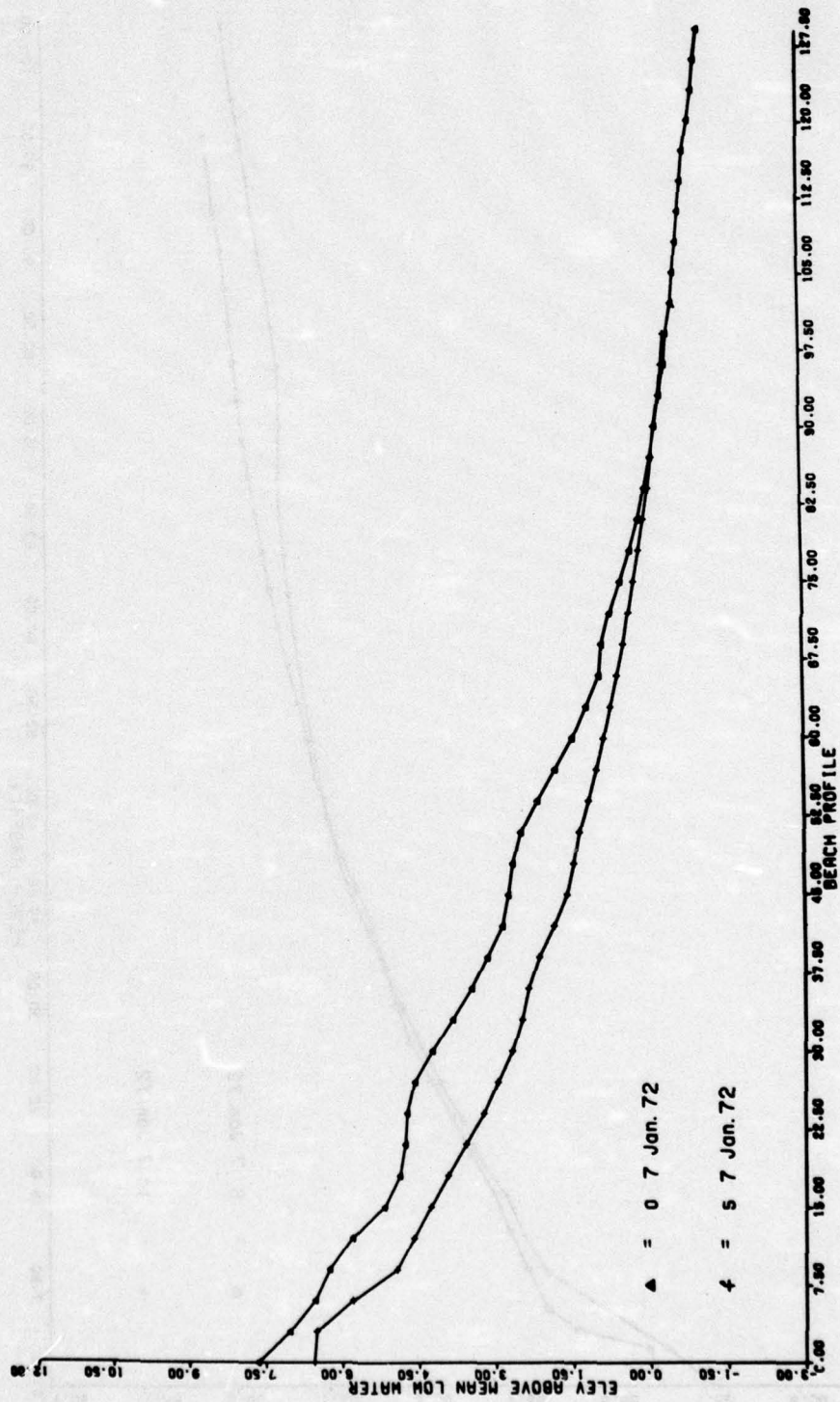
Figure 62. Profiles PL-0 and PL-5, 7 January 1972.
