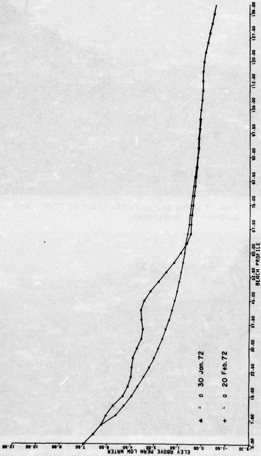
Figure 76. Profile PL-0, 30 January to 20 February 1972.
