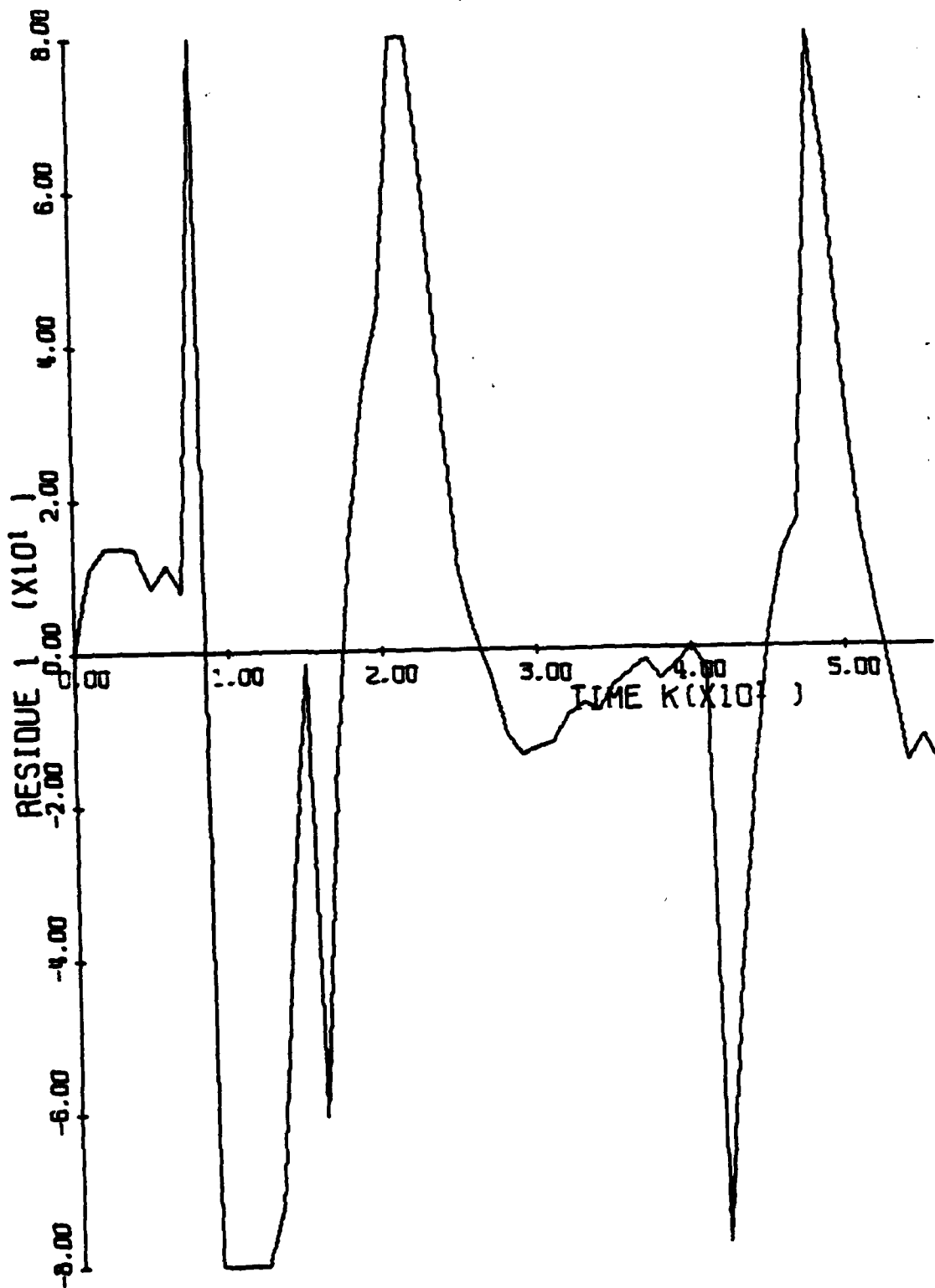
FIGURE 10: Residue 1 vs. Time. Q = .01I , R = I .
