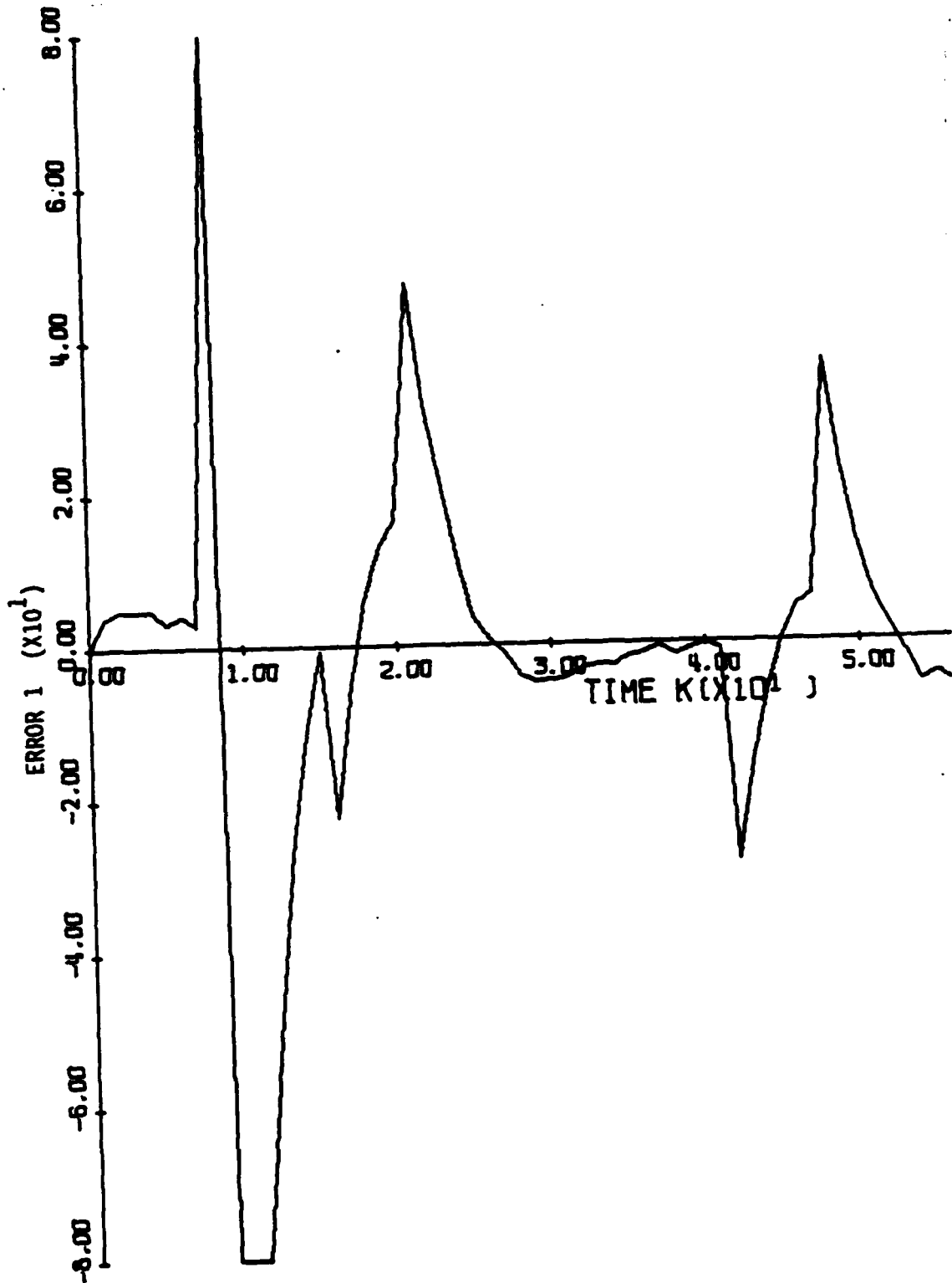
FIGURE 12: Error 1 vs. Time. Q = .01I , R = I .
