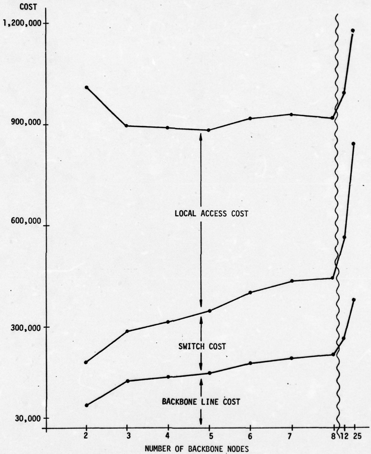
FIGURE 8: TRAFFIC - 10 TIMES HARDWARE COST - NOMINAL
