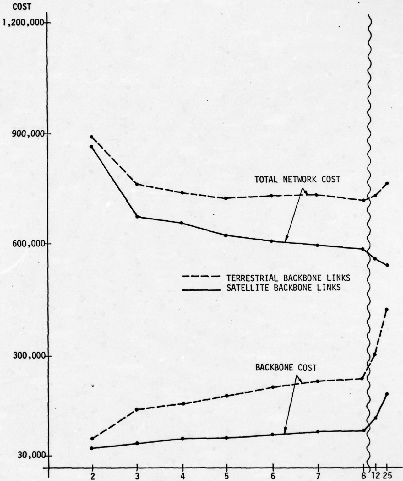
NUMBER OF BACKBONE NODES FIGURE 26: TRAFFIC - 10 TIMES SATELLITE CHANNEL COST - 1/2 HARDWARE & GROUND STATION COST - 1/10
