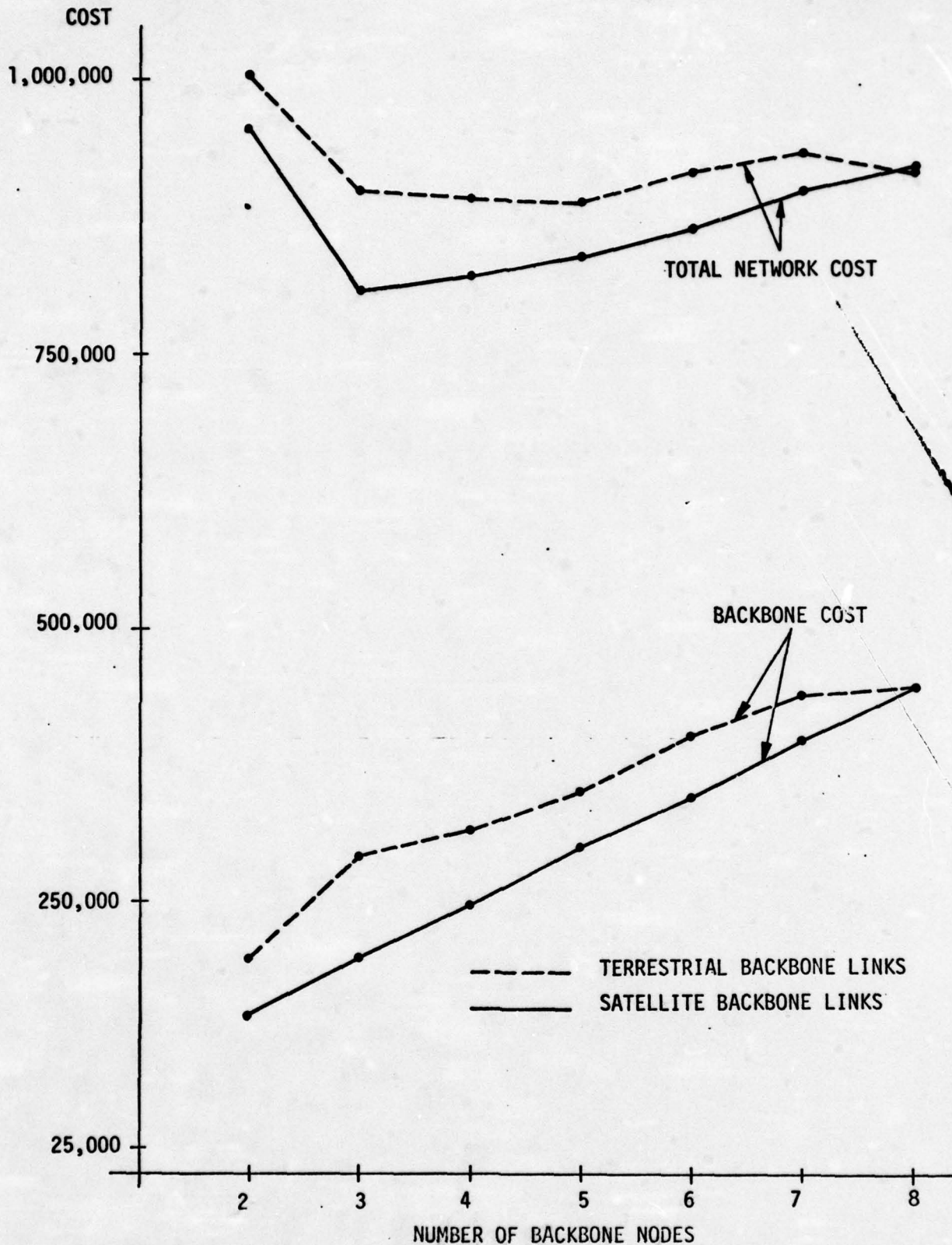
FIGURE 21: TRAFFIC - 10 TIMES
