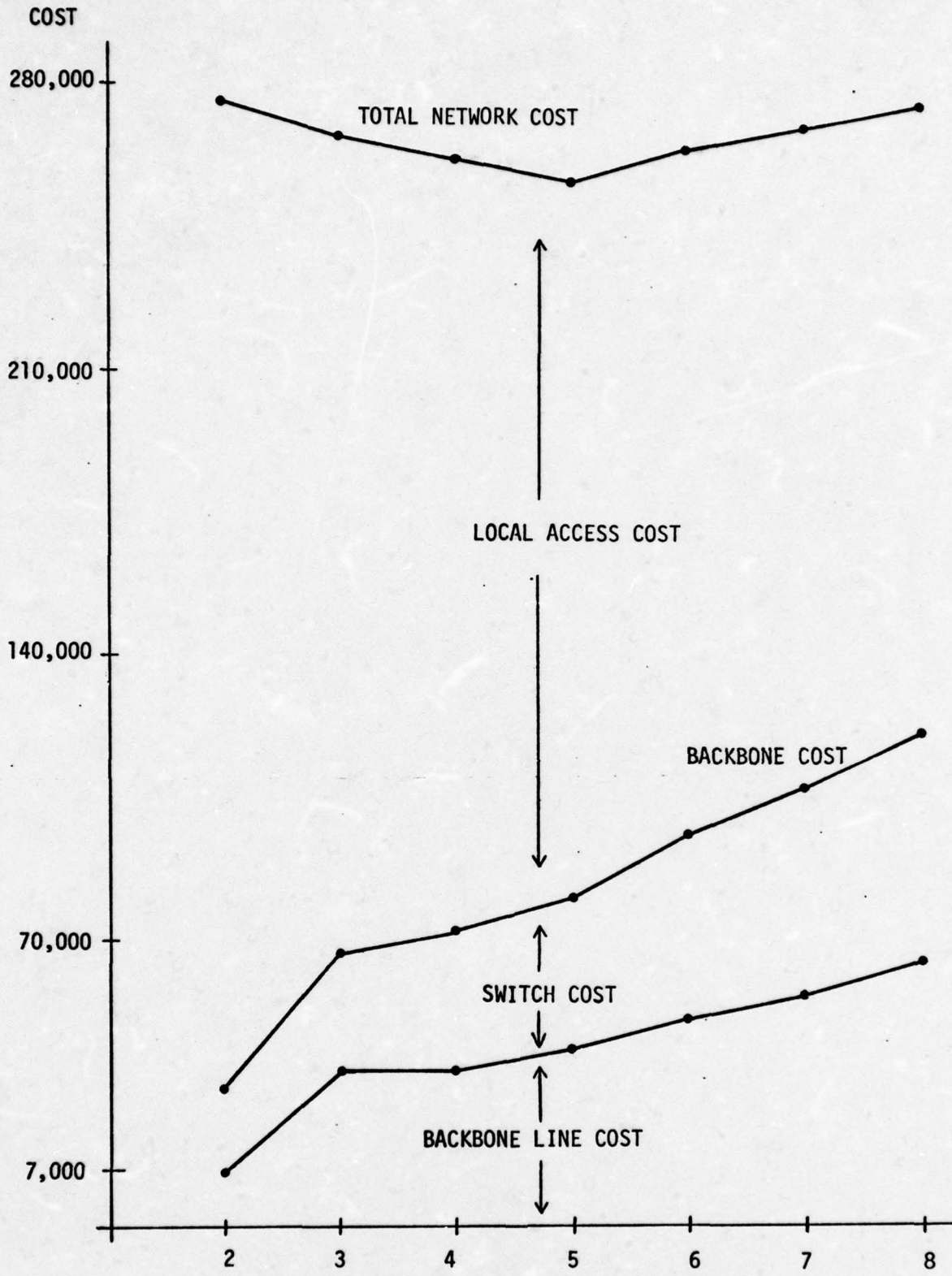
NUMBER OF BACKBONE NODES FIGURE 4: TRAFFIC - NOMINAL HARDWARE COST - NOMINAL 6.28
