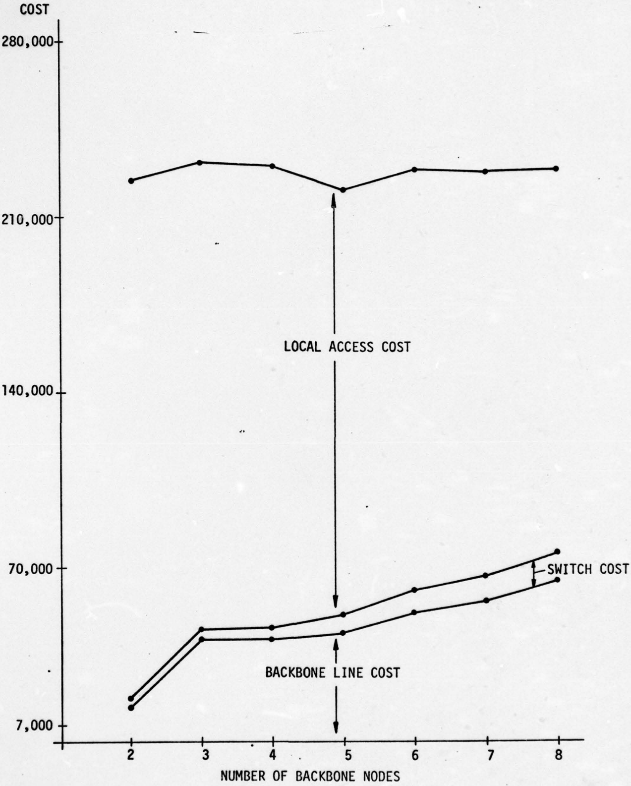
FIGURE 6: TRAFFIC - NOMINAL HARDWARE COST - 1/5
