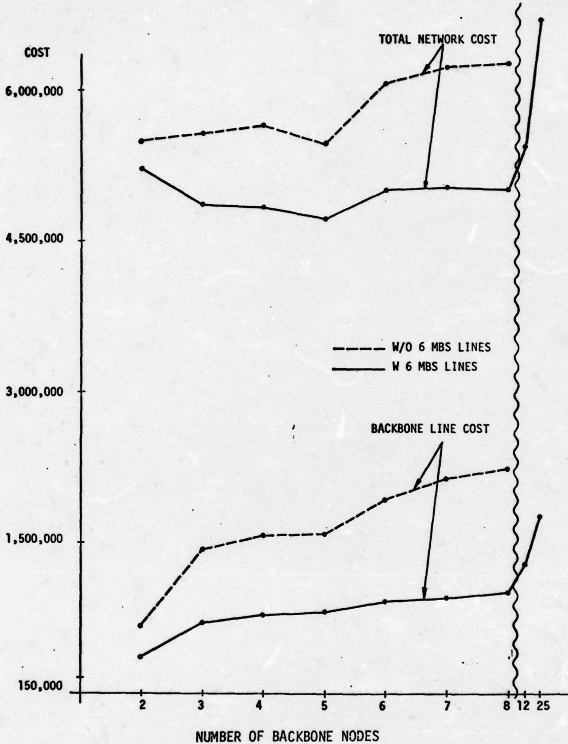
FIGURE 28: TRAFFIC - 100 TIMES HARDWARE COST - NOMINAL W 6 MBS LINES
