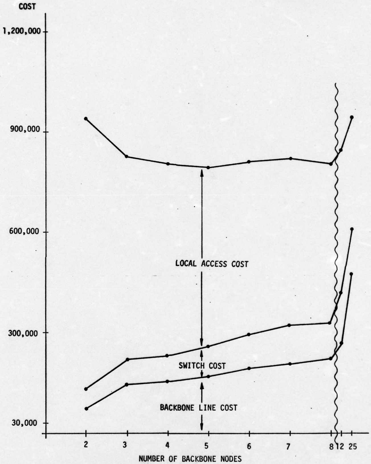
FIGURE 9: TRAFFIC - 10 TIMES
