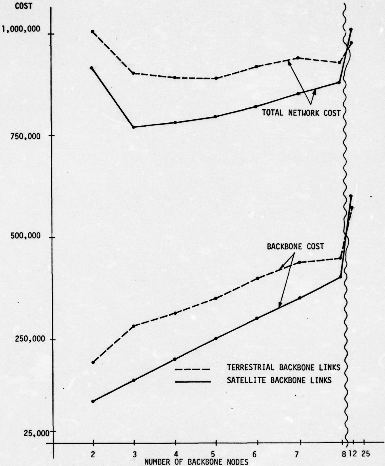
FIGURE 23: TRAFFIC - 10 TIMES SATELLITE CHANNEL COST - 1/10
