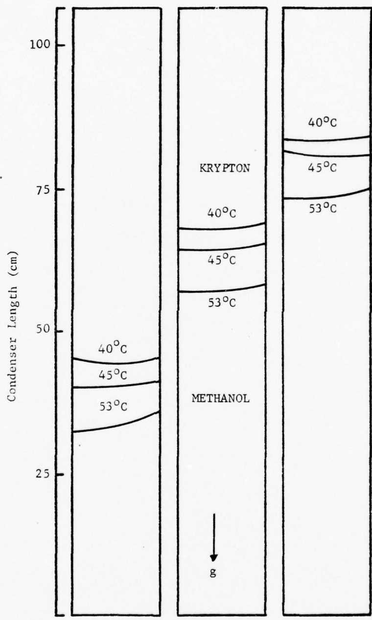
Liquid Crystal Isotherms - Vertical 6.17 \times 10^{-4} kg Krypton Figure 14
