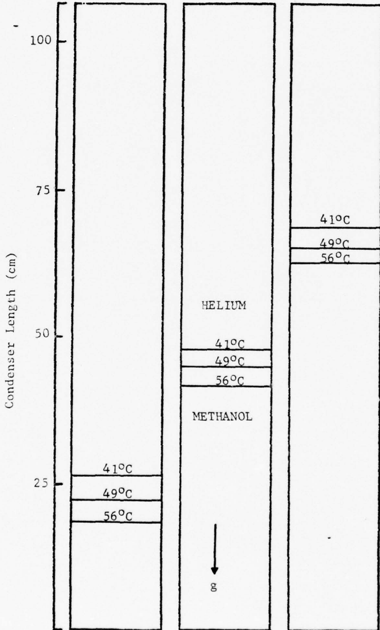
Liquid Crystal Isotherms - Vertical 1.82 \times 10^{-4} kg Helium - Batts' Results Figure 25
