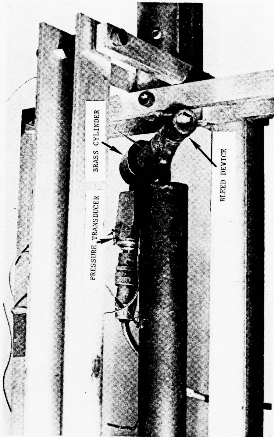
Photograph of Condenser End of Heat Pipe
