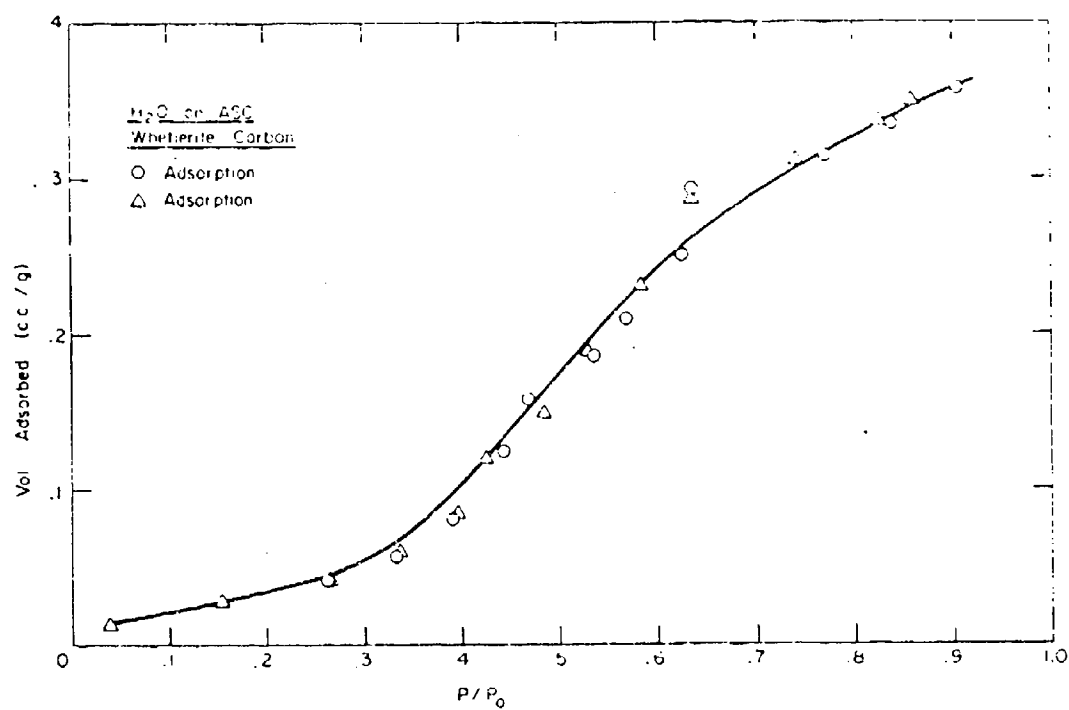
Figure 2. H 2 O on ASC Whetlerite Carbon
