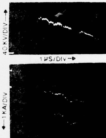
FIGURE 3. GUN VOLTAGE AND GUN STEM CURRENTS WITH MARX GENERATOR EXCITATION
