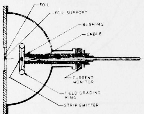
FIGURE 2. GUN CROSS SECTION
