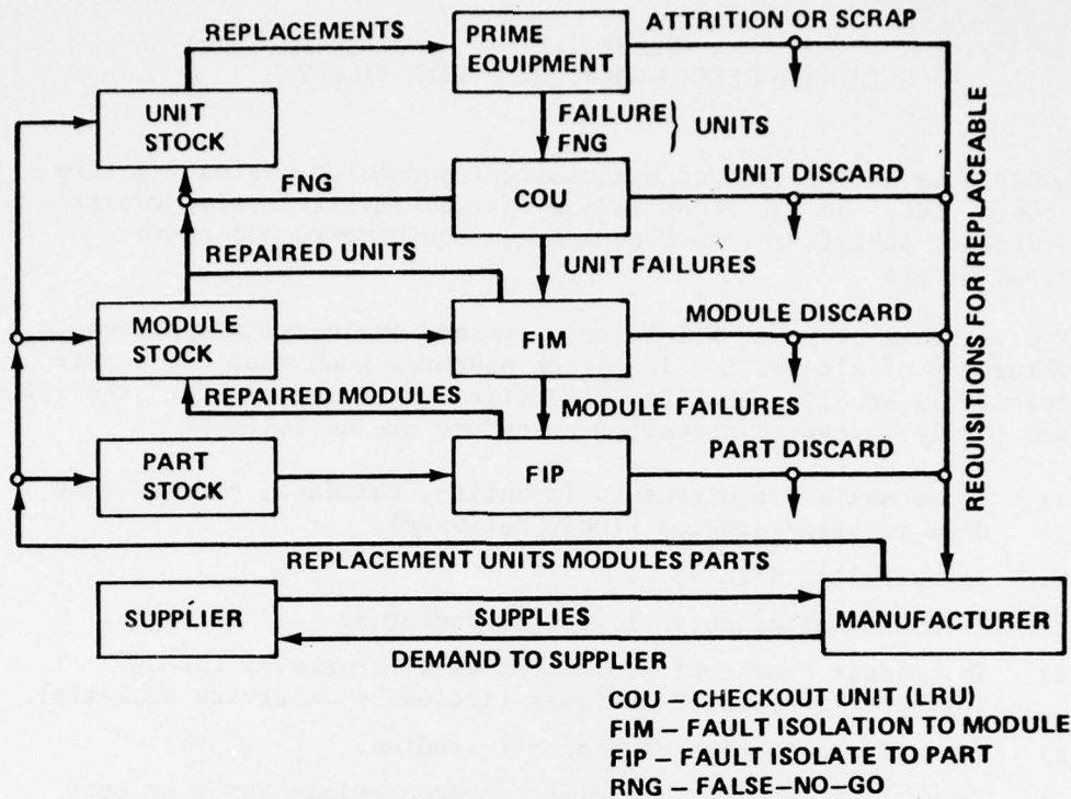
Figure 1. Basic LOCAM 5 repair flow framework.
