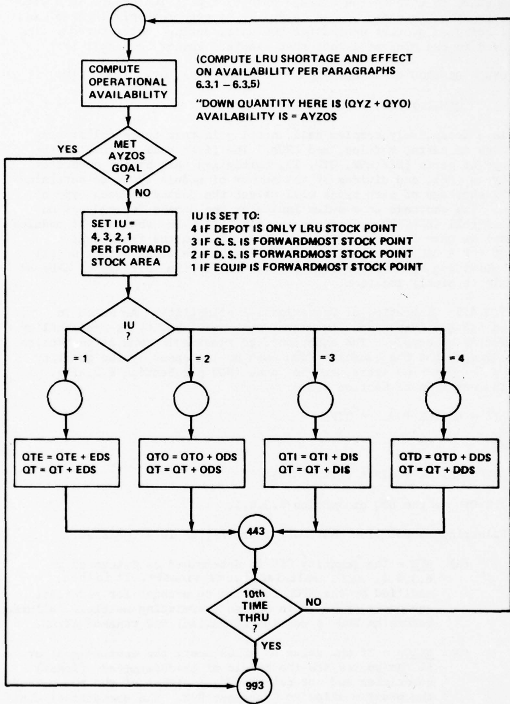
Figure 29. Operational availability.
