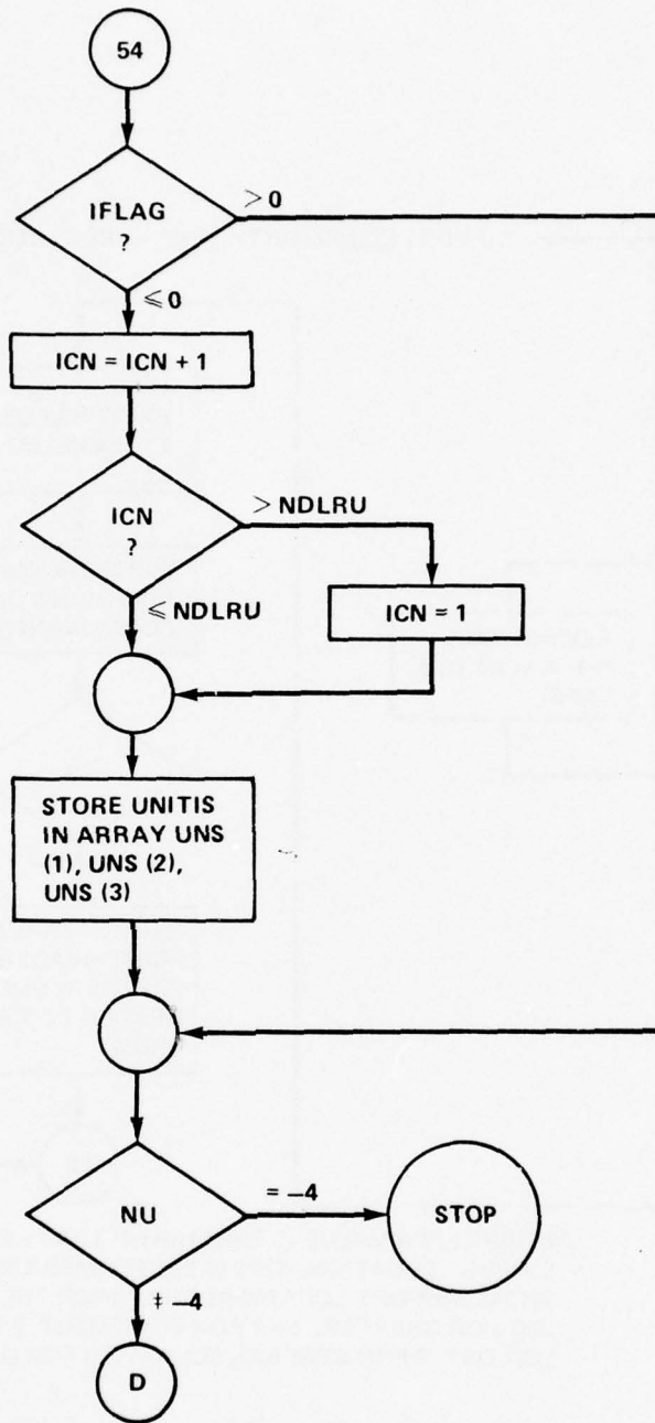
Figure 9. Control of summary total accumulation (Block "C" of Figure 5).
