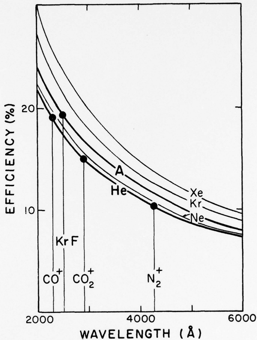
Figure 1: Graph showing the limiting efficiencies as functions of wavelength for excimer and charge transfer lasers operating in inert gases. Filled circles represent systems of current interest.
