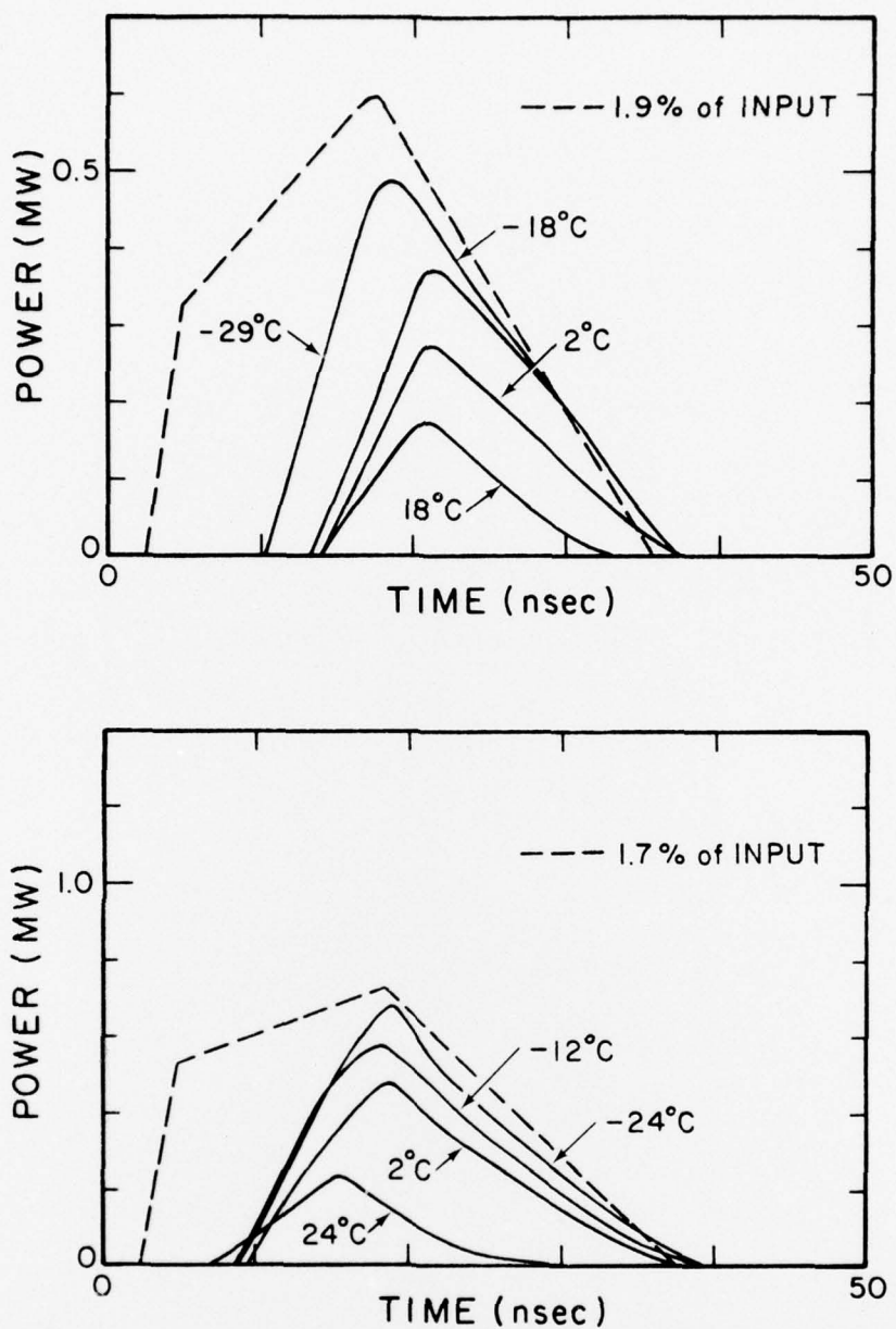
Figure 6: Plot of the time-resolved laser power emitted at 4278\text{\AA} from an electron beam discharge into 7.7 atm pressure of helium containing 15 torr of \text{N}_2 at the gas temperatures shown. The dashed curves show the time dependence of a constant fraction of the corresponding input power deposited in the laser cavity. (a) Upper curves: Data for nominal 15KA e-beam current, (b) Lower curves: Data for nominal 20KA e-beam current.
