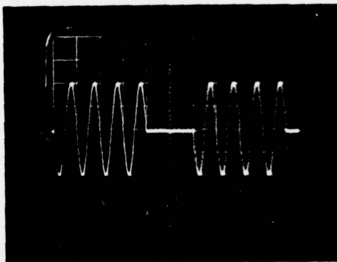
Figure 7. IM SIGNAL MODULATED BY A SINUSOID. f_c = 200 \text{ kHz} , j = 4 , k = 2 , l = 6 , x_0 = 0 , and -0.04 \leq x(t) \leq 0.04 (9.8 \text{ } \mu\text{s} \leq T_x \leq 10.2 \text{ } \mu\text{s}) .
