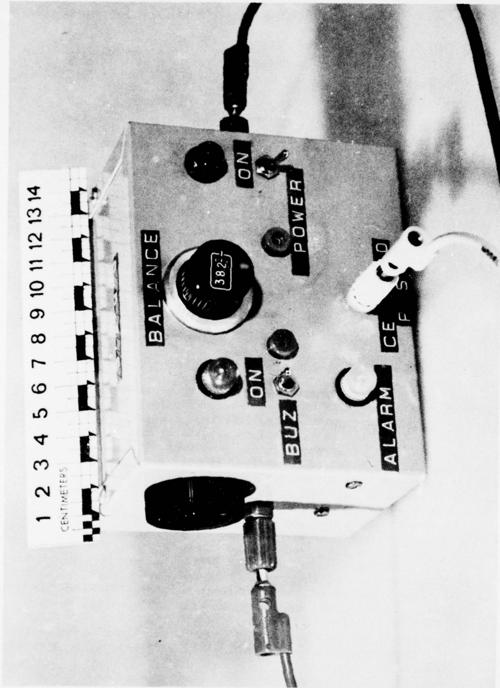
Fig. 1: Battery Alarm Unit - Experimental Model
