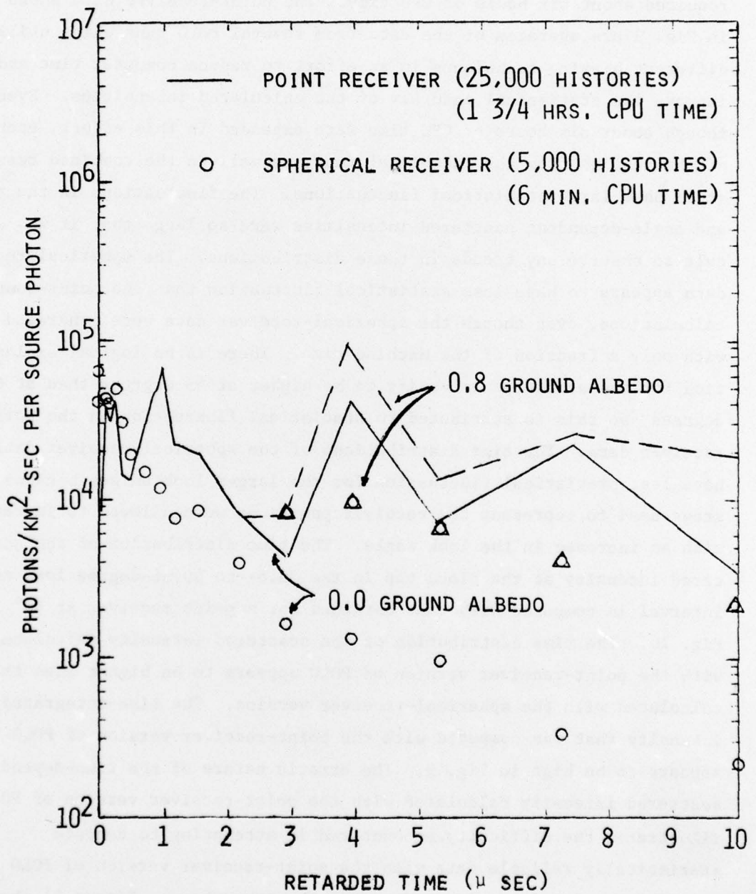
Fig. 10. Scattered Intensity at Top of 5 Mean-Free-Path Thick Stratus Cloud for a Look Angle of 40 Degrees
