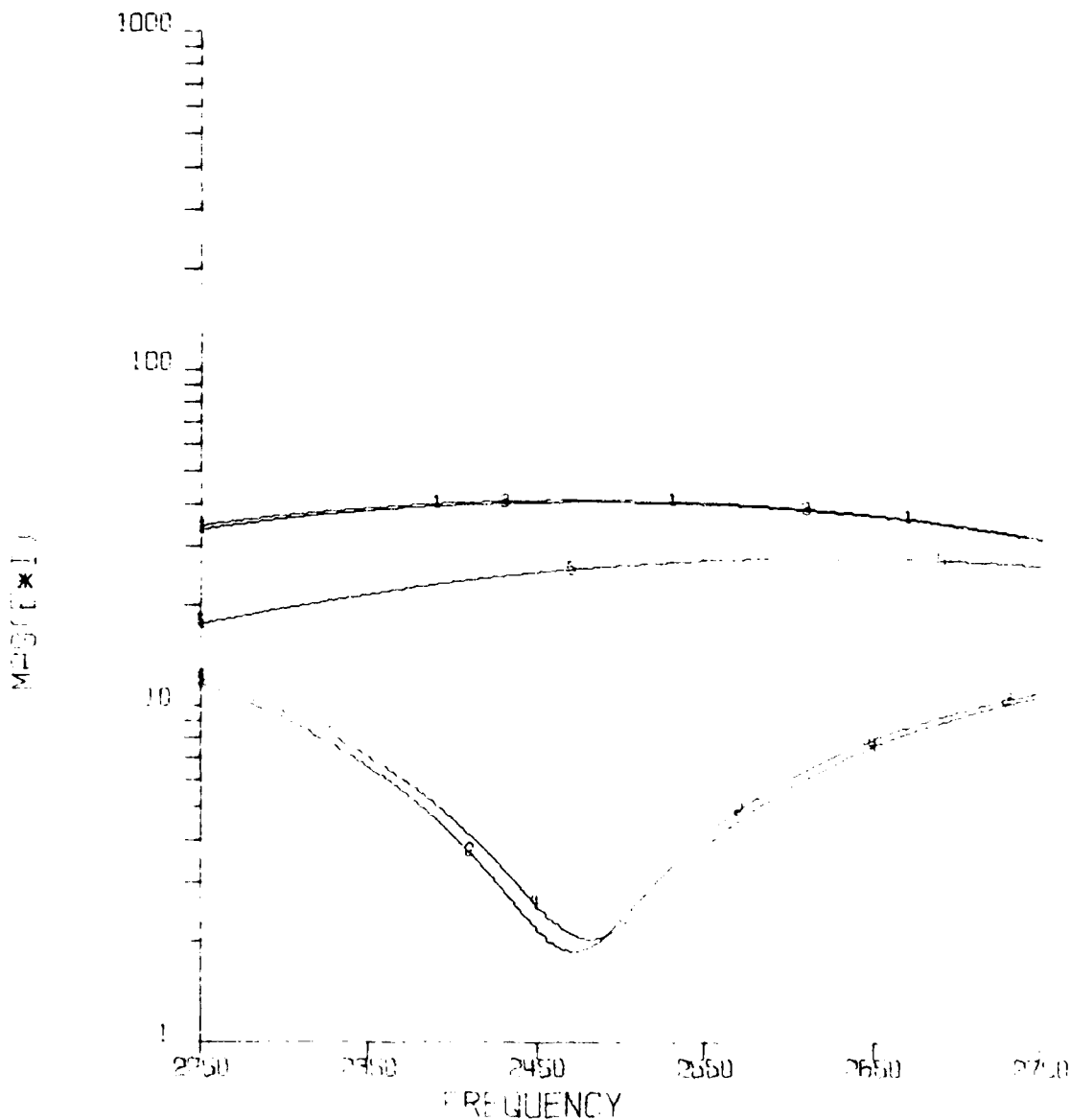
MAG (T * I) VERSUS FREQUENCY
