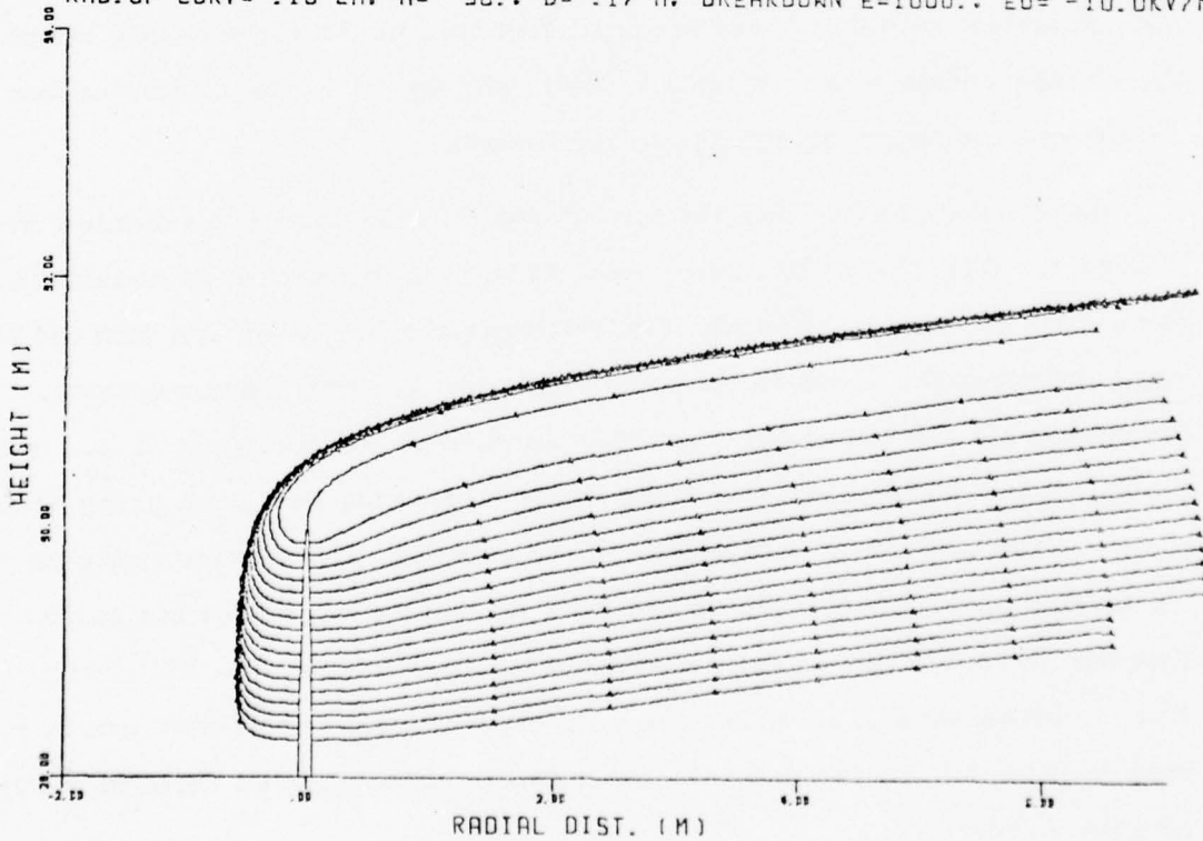
Figure 7. Ion Movement under Horizontal Winds Showing Maximum Boundary of Ion Cloud
