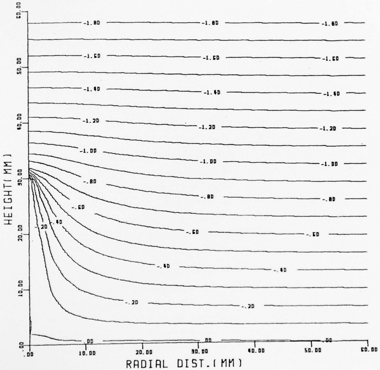
Figure 6. Equipotential Lines around a Sharp Point on Top of a Rounded Structure
