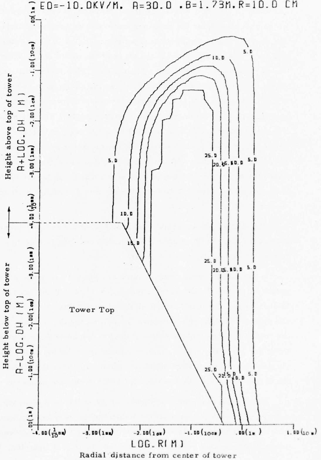
Figure 8. Expansion of Ion Cloud into Wind
