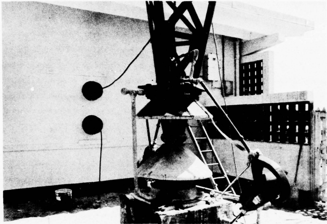
Figure 44a. The base of the USCG, Loran C antenna at Jupiter, Florida showing the insulated base, spark gaps and transmitter leads
