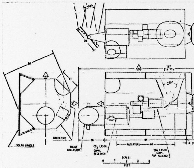
Fig. 1. Satellite Configuration.
